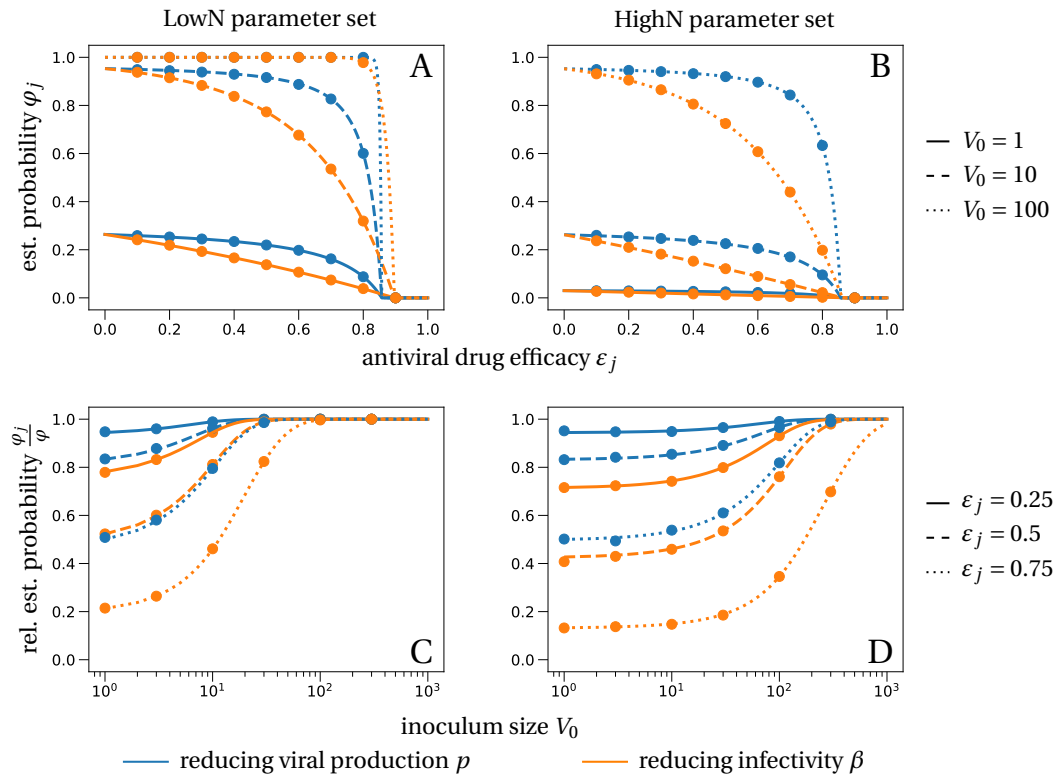
Figure 2: Establishment probability of the virus under different antiviral drugs, efficacies and various inoculum sizes V_0 . The lines in panels A and C correspond to the theoretical establishment probability under the assumption that target cell numbers are constant, adapted to the two modes of action (reducing viral infectivity (5) in orange and reducing viral production (6) in blue). The lines in the bottom panels represent the relative probability of establishment normalized by the establishment probability in the absence of treatment from (4), i.e. \varphi_j/\varphi . The theoretical predictions align well with the averages obtained from 100,000 individual based simulation of the within-host model described in system (3), in which target cell numbers are allowed to vary. Parameter values are given in Table 1.
