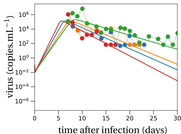
Figure 1: Deterministic within-host dynamics in four SARS-CoV-2 infected patients. Model predictions using the target cell limited model in four typical patients of Young et al. (2020), with a mean R_0 of 7. Parameter values are given in Table S2 in the Supplementary Information.
