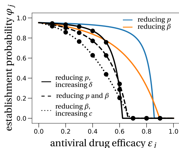
Figure 3: The effect of prophylactic combination therapy on the establishment probability.
