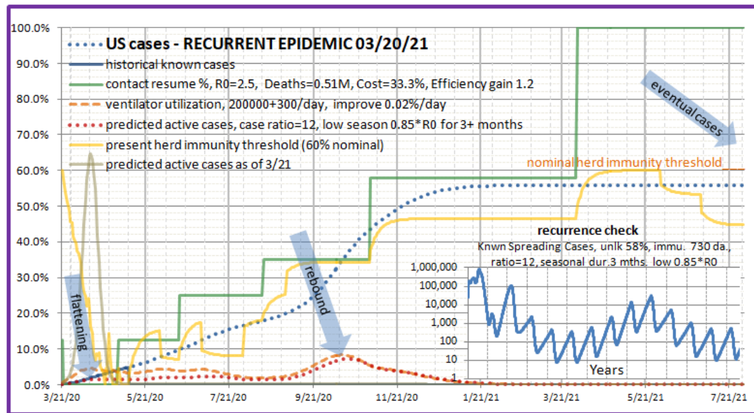
Figure 16. US cases with 15% seasonality adjustment, reduced mortality over 6 month by half, and 1.2x economic efficiency
