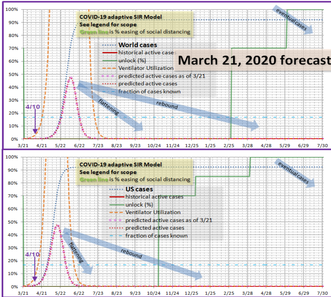
Figure 3. Initial projection for world and US based on data through 3/21.
