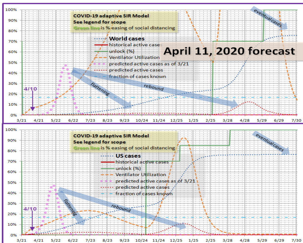
Figure 5. Flattening progress for world and US based on data through 4/11.
