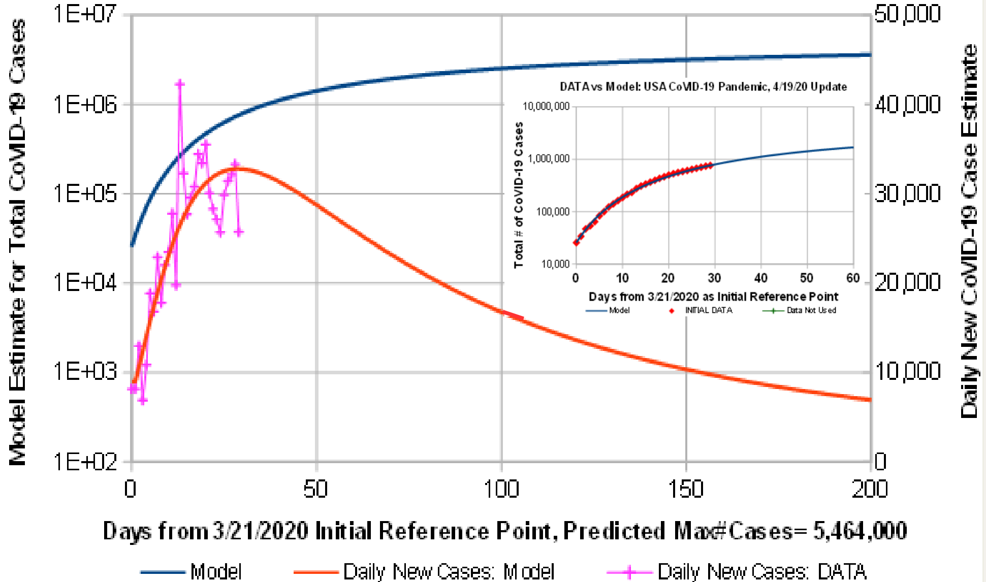
Figure 3: USA Model Predictions. To allow better mitigation predictions, only data after mid-March 2020 was included, when several Governors instituted mandatory lockdowns.
