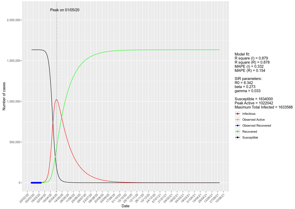
COVID-19 SIR model Malaysia, Pre MCO - 1 week MCO Projection from data: 2020-03-01 to 2020-03-24
