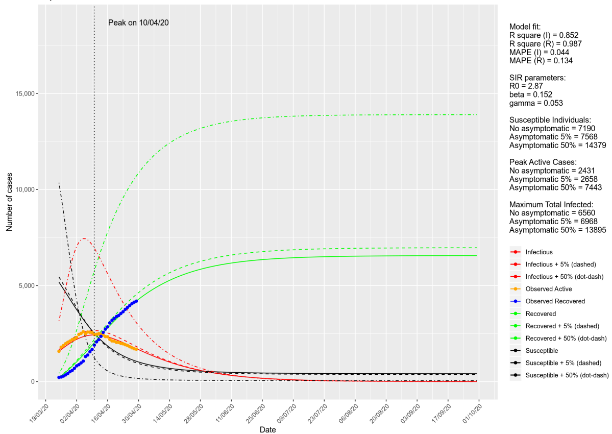
COVID-19 SIR model Malaysia, MCO week 2 -> Today Projection from data: 2020-03-25 to 2020-04-29
