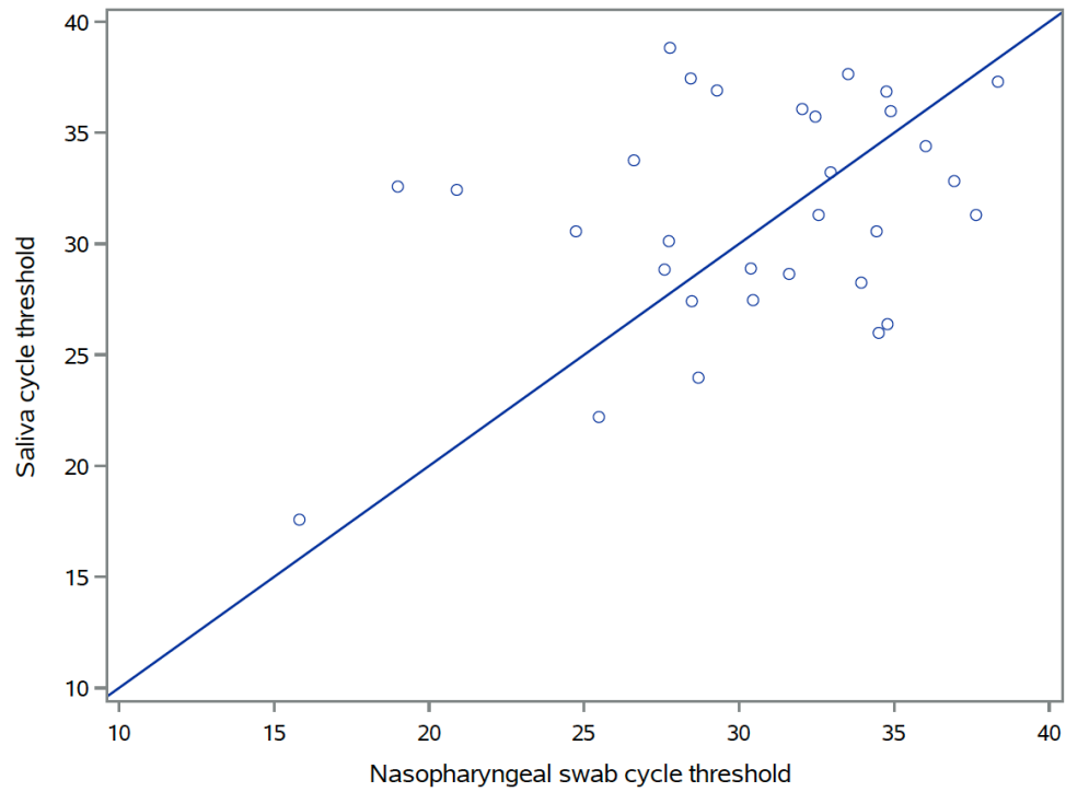
Figure. Nucleocapsid (N) gene cycle thresholds for nasopharyngeal swabs and saliva in pairs where both were positive for SARS-CoV-2 RNA (N=31).
