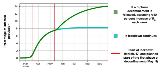
Fig. 3. Predicted number of infected proportion of France from February 15, 2020 to September 21, 2020; considering a scenario, where quarantine time reproduction number grows by 10% each week, during 3 weeks following lockdown lift.
