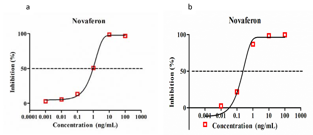
Figure 1. Concentration-effect relationship of the inhibition of Novaferon on SARS-CoV-2 replication. The experiments were done in triplicates. a. inhibitory effects of Novaferon after virus infection; b. inhibitory effects of Novaferon before virus infection.
