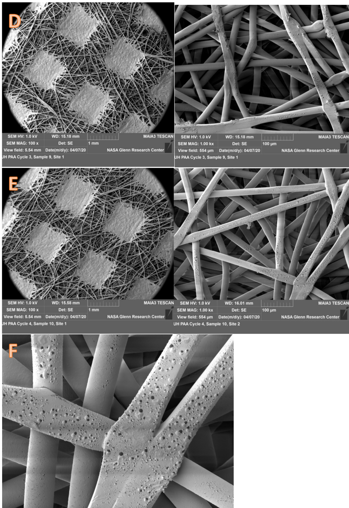
Legend: Figure 6 shows SEM images of the outer layer of the N95 mask under 100x (images in the left column) and 1000x magnification (images in the right column. A (control), B though E indicate multiple cycles of PAA treatment from 1-4. Note increase bubbling on the fibers after PAA exposure. Magnified image of bubbling on fibers (6F)
