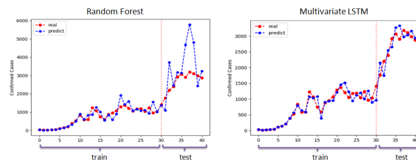
Figure 8: Comparison of the worst and the best performing models in correct following of the training set and accurate prediction of the test values.
