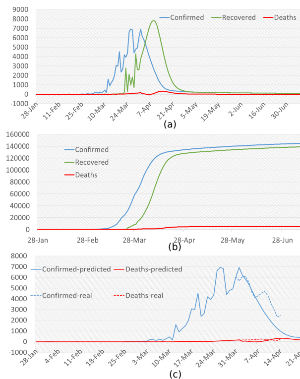
Figure 12: Forecasting confirmed, death, and recovered values for Germany using M-LSTM method for (a) daily and (b) cumulative values, and performance of the forecasting after April 2 compared to real reported values.
