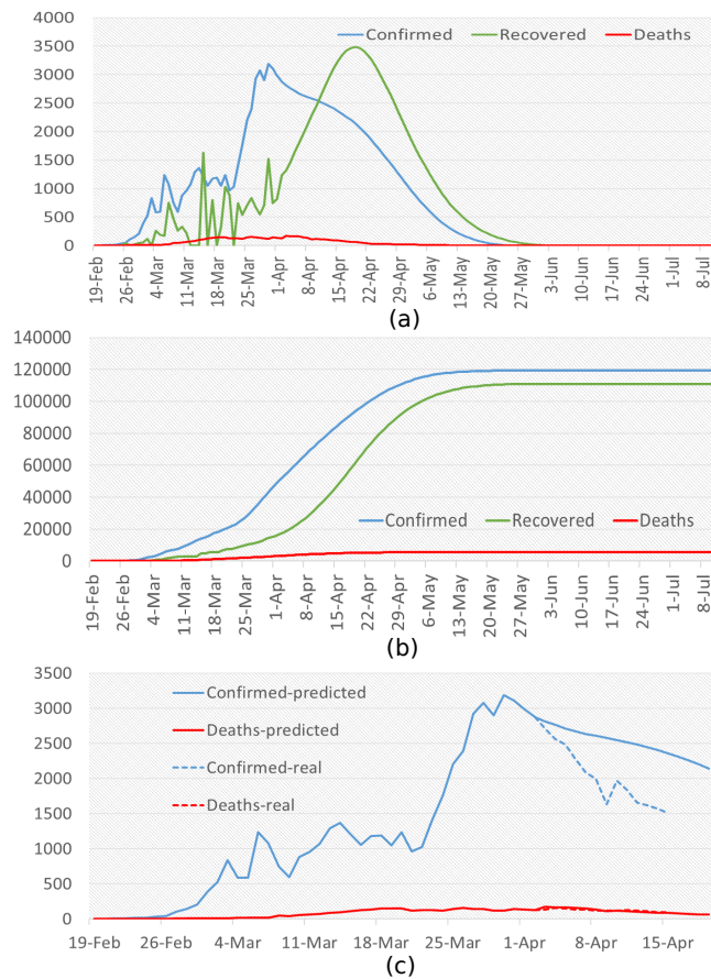
Figure 9: Forecasting confirmed, death, and recovered values for Iran using M-LSTM method for (a) daily and (b) cumulative values, and performance of the forecasting after April 2 compared to real reported values.
