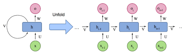
Figure 5: RNN model
