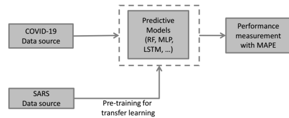
Figure 2: COVID-19 disease prediction models.
