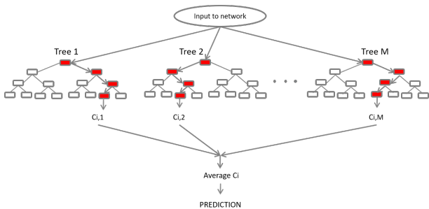
Figure 3: The overall diagram of a RF.
