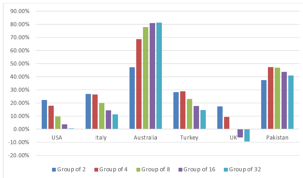
Graph 1: Showing how many tests in percentage, every country can save to tests a population of 10,000
