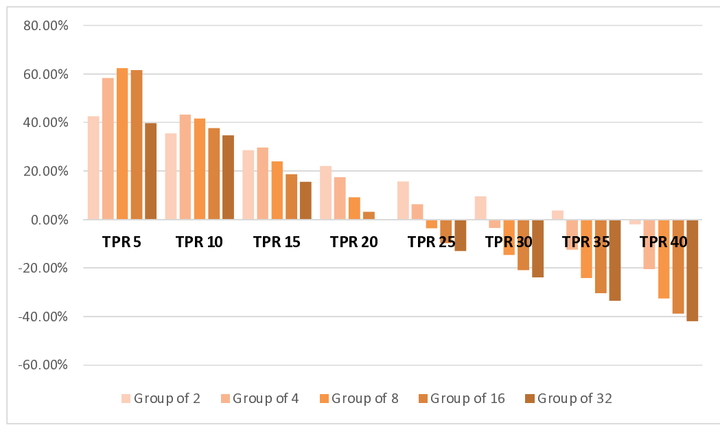
Graph 2: Showing how many tests in percentage, one can save to tests a population of 10,000
