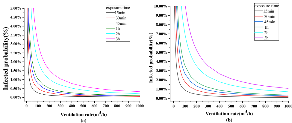
Figure 3. Infected probability with different ventilation rate during different exposure time (a) q=14/h (b) q=48/h (with mask)
