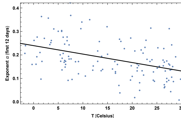
Figure 4: Exponent \alpha for each country vs. average temperature T , for the relevant period of time, as defined in the text, for the extended set of 125 countries. We show the data points and the best-fit for the linear interpolation.
