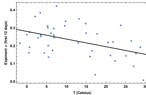
Figure 1: Exponent \alpha for each country vs. average temperature T , for the relevant period of time, as defined in the text, for the base set of 42 countries. We show the data points and the best-fit for the linear interpolation.
