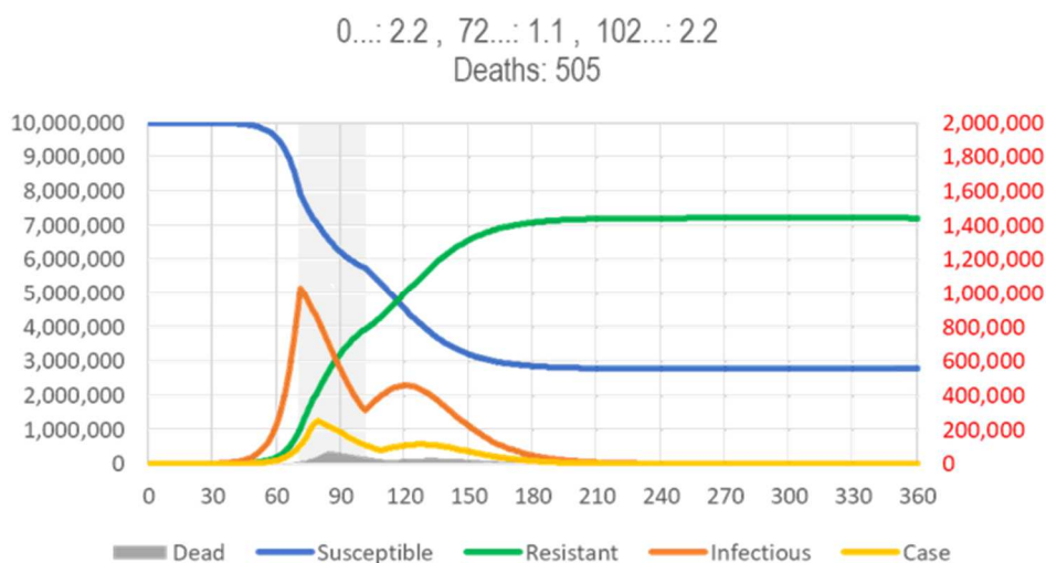
Fig 13: SIR Model of SARS, Window of Opportunity for Maximal Reduction of Total Deaths. (see Fig 3 for legend). The gray area indicates the period where containment can have the most impact on total number of deaths. However, the epidemic is not eradicated. (spreadsheet for model calculations available from https://app.box.com/s/pa446z1csxcvfksgj13oohjm3bjg86ql )
