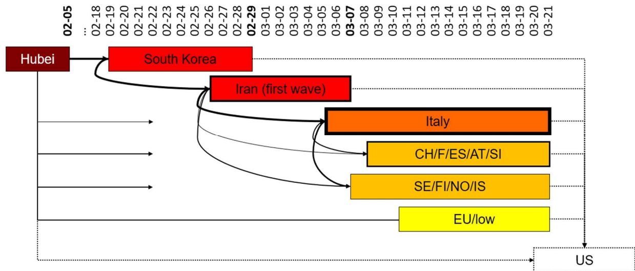
Fig 16: Hypothetical virus transmission pathways. Connection width: number of contacts, box colors: infectiousness, box borders: lethality, dotted connections/borders: unknown. The end date of a box indicates the date of peak incidence, if known (bold date).
