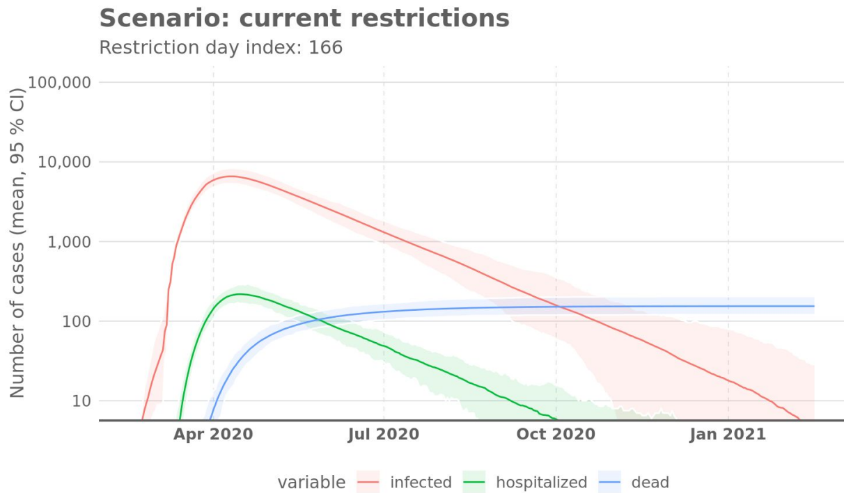
Figure S-1. Numbers of cases of the scenario with permanent 50% mobility restriction (which is the situation in Finland on 2020-04-01), mean and 95% confidence intervals of the random variation.
