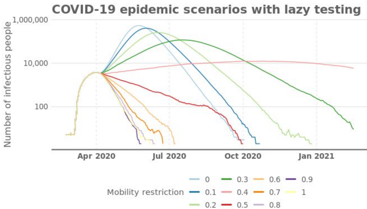
Figure 4. Number of active (infective) COVID-19 patients with different mobility restrictions and lazy testing (only severe cases are tested).
