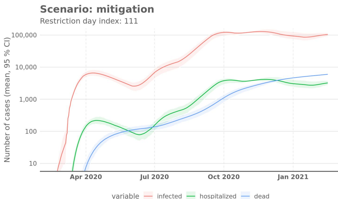
Figure 7. Numbers of cases in a scenario under the mitigation strategy. It contains aggressive building of hospital capacity and mobility restrictions (varying between 30–40%) just enough to prevent shortage in the capacity (a common suggestion in Finnish discussion in mid-March, 2020). Mean and 95% confidence intervals of the random variation produced by the modeling approach. They do not incorporate parameter uncertainties.
