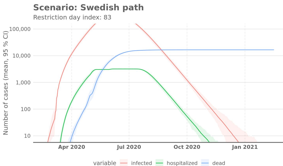
Figure S-2. Numbers of cases of the scenario with permanent 25% mobility restriction (which was the situation in Sweden on 2020-04-01 [Google, 2020]), mean and 95% confidence intervals of the random variation.
