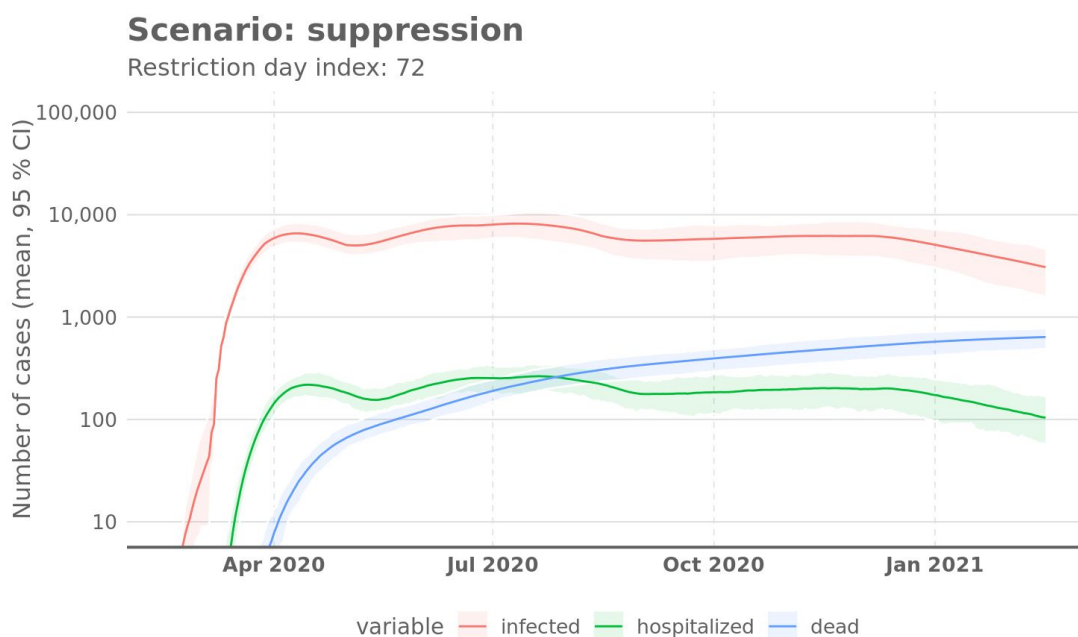
Figure 8. Numbers of cases in a scenario under suppression strategy. It contains initially 50% mobility restriction (the situation in Finland on 2020-04-01) but then loosening restrictions to 20–25% as aggressive testing and tracing becomes effective. Mean and 95% confidence intervals of the random variation by the modeling approach. They do not incorporate parameter uncertainties.
