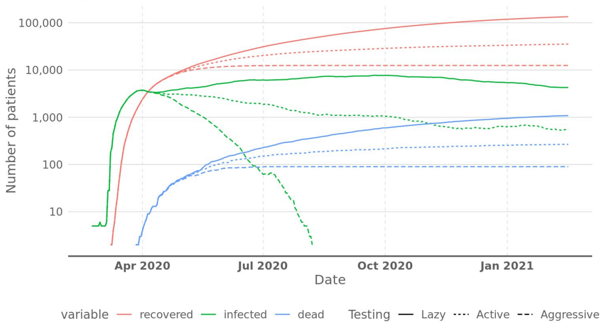
Figure 6. Number of active, infectious cases, recovered, and COVID-19 deaths as a function of time, with 41% mobility restriction (resulting in 137 RDI) and one of the testing policies applied permanently since April 6th, 2020.
