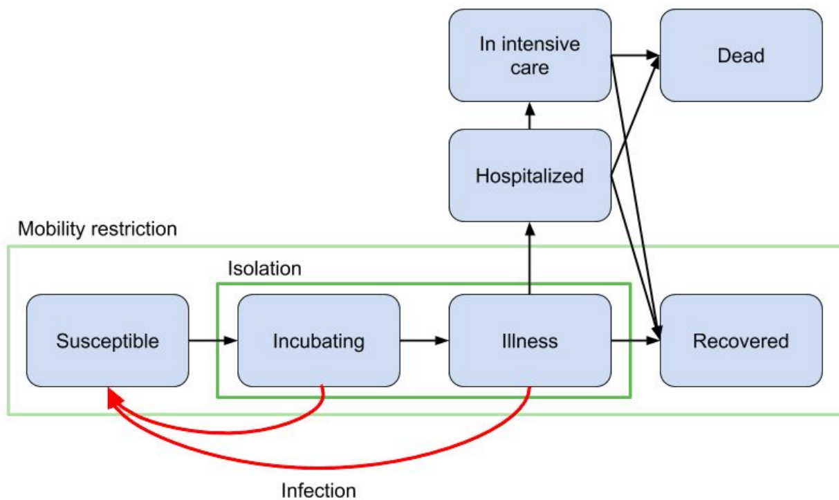
Figure 1. Diagram of the coronavirus agent model. Blue nodes: different states of the agents. Black arrows: transitions between the states. Red arrows: infection pathways. Green boxes: targeted (isolation) and broad (mobility restriction) population subgroups under varying degrees of social isolation. Incubating state contains people that already have the virus and may spread it but the actual illness (i.e., symptoms) has not yet started (see Table 1). In this model, the “exposed” state is treated implicitly, and the “infectious” state is divided into four sub-states. Thus, they are not shown here as state names.
