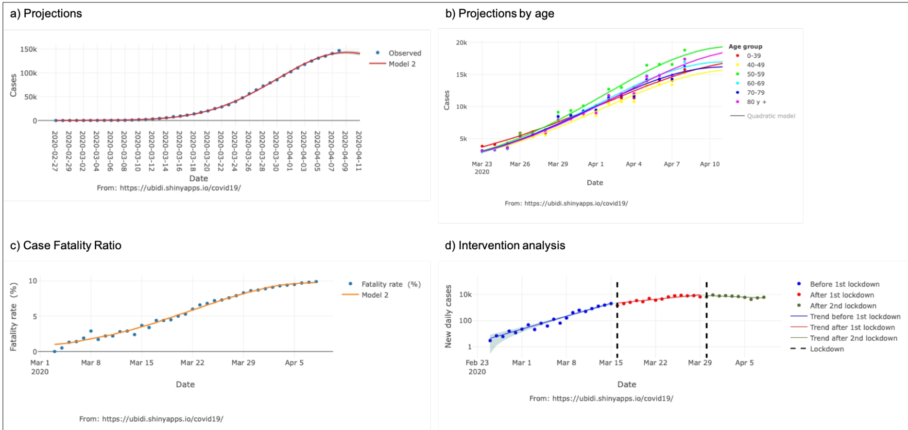
Figure 2. Standard output display of the COVID19-Tracker application (results updated to April 8th, 2020), for trend analysis and its 3-day projection at the national level (a) and by age group (b), of the fatality rate (c), and intervention analysis to evaluate the effect of alarm states on incident data (d).
