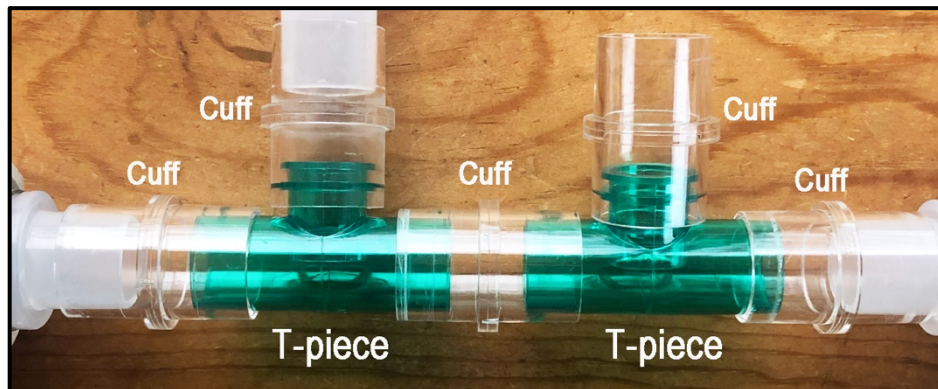
Figure 6: T-piece connections. Two T-pieces are connected using an interposed cuff, and then cuffs are attached to all outlets to provide connections to the circuit.
