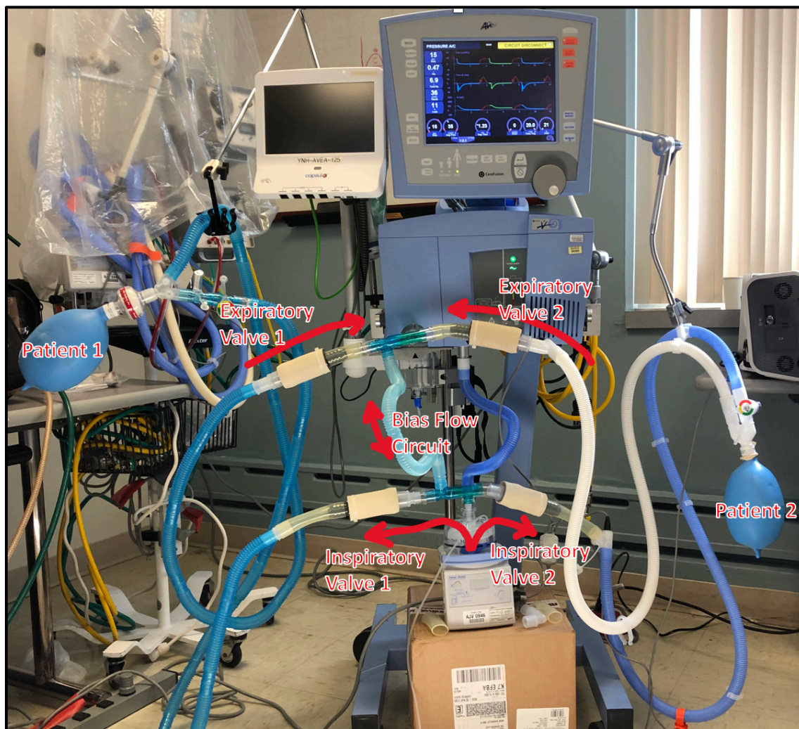
Figure 1: Photograph of the PReVENTS Ventilator Splitting Design. Two patients are simulated in this setup. Four pressure-gated inline valves, derived from PEEP valves for bag-valve-mask assemblies, are in the two-patient circuit. Two inspiratory valves control PIP to the two patients. Two expiratory valves control PEEP to the two patients. A “Bias Flow” circuit provides a bypass flow path parallel to the two patient paths to prevent automated ventilator alarming due to high circuit resistance, an artifact which is intrinsic to the placing of in-line pressure-gated valves. It should be noted that this bypass circumvents a set of alarms which clinicians may be used to relying on during patient care (see below).
