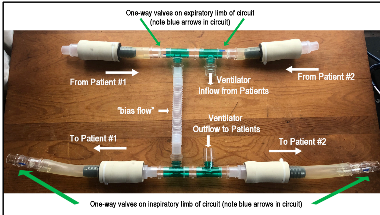
Figure 7: Simplified Overview of the PReVentS Circuit. Flow into and out of the ventilator is shown, next to a "bias flow" circuit which prevents false triggering of the ventilator occlusion alarm. The placement of in-line pressure-gated (PEEP) valves is shown for 2 patients, along with gas flow paths through the in-line valves. Locations of one-way valves are shown in inspiratory and expiratory limbs.
