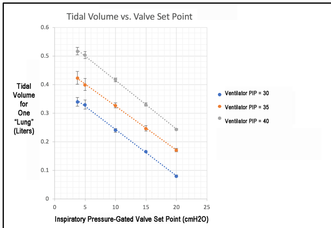
Figure 11: Impact of Inspiratory pressure-gated valve setting on tidal volume. Tidal volumes shown for 3 different settings of ventilator PIP. Data are from N=3 replicates. Dotted lines are linear fits.
