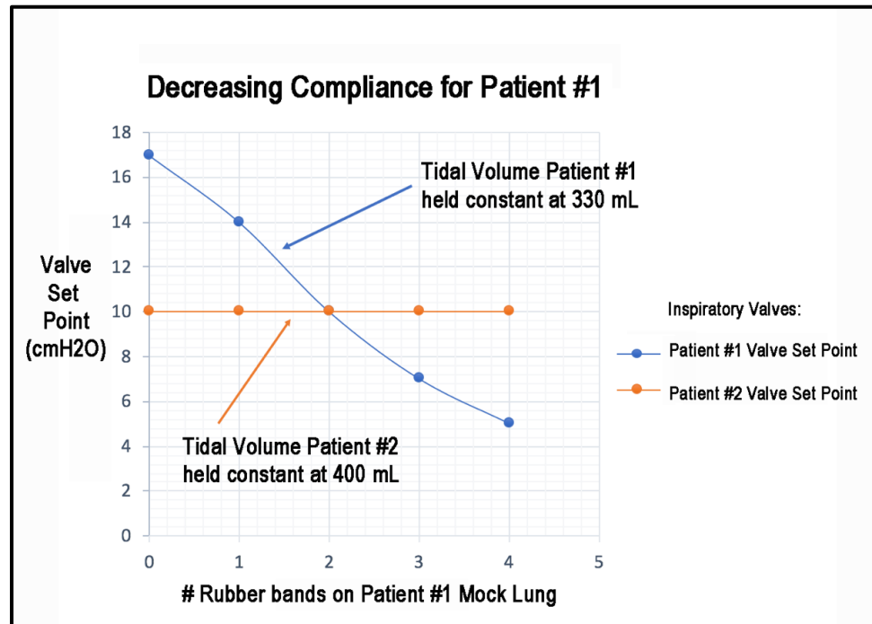
Figure 13: Impact of Decreasing Lung Compliance in One Patient. Compliance of mock lung for Patient #1 was decreased by sequentially adding rubber bands to the outside of the rubber ventilator bag. As Patient #1 compliance decreased, tidal volume could be maintained for Patient #1 by adjusting the pressure-gated valve for Patient #1 on the Inspiratory limb. During these maneuvers, tidal volumes for Patient #2 were not affected.
