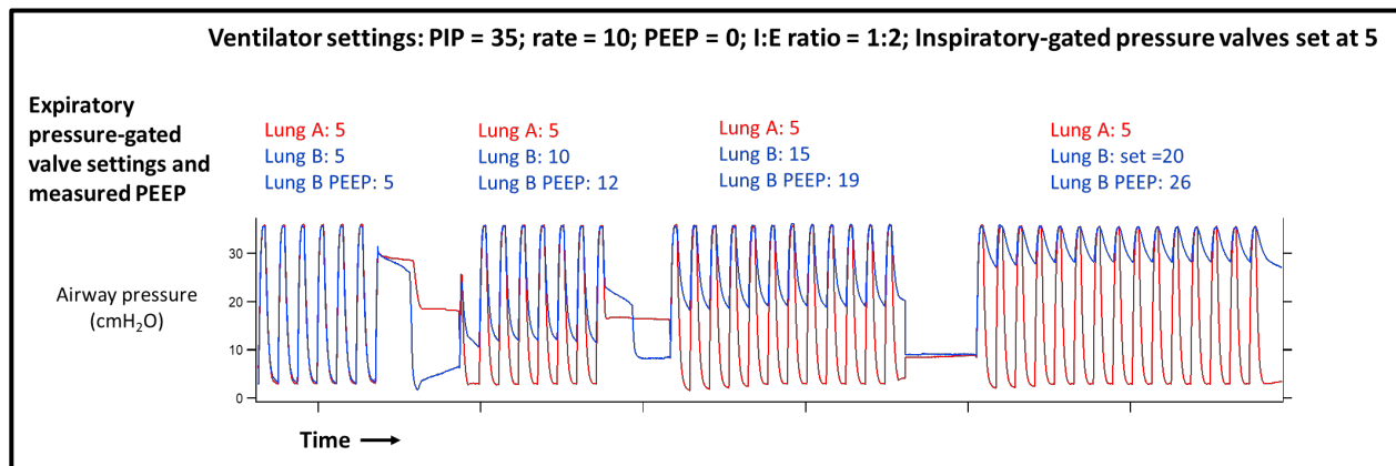
Figure 14: Impact of increasing the set point of the expiratory pressure-gated valve for one patient in the PReVentS circuit. By adjusting the set point of the expiratory pressure-gated valve for Lung B , we can selectively increase the amount of Positive End-Expiratory Pressure (PEEP) for Lung B , while not affecting Lung A . Data suggest the potential for “breath stacking” as indicated by higher levels of measured PEEP for Lung B . Patient #1 corresponds to Lung A , while Patient #2 corresponds to Lung B . Expiratory valve pressure settings are in cmH 2 O.
