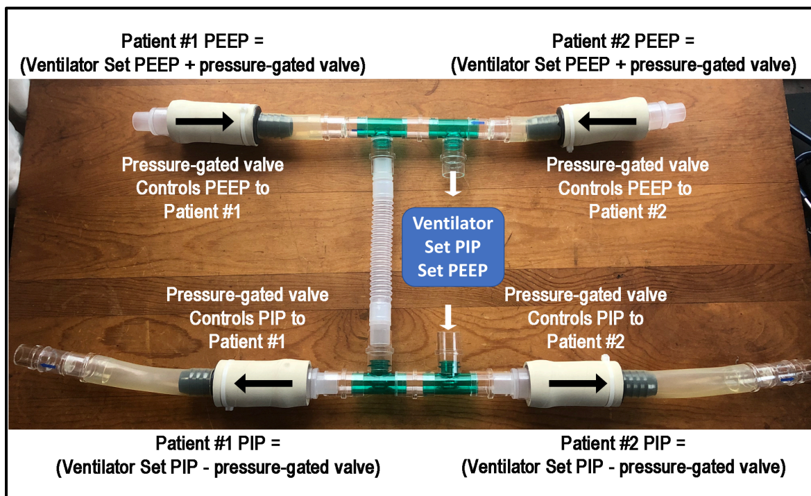
Figure 8: Flow paths of ventilation from the ventilator to each patient. The ventilator provides a single setting of PIP and PEEP to the circuit. The inspiratory limb of the circuit (bottom of figure) contains two in-line pressure-gated valves that control the PIP to patients #1 and #2. The expiratory limb of the circuit (top of figure) contains two in-line pressure-gated valves that control the PEEP to patients #1 and #2.
