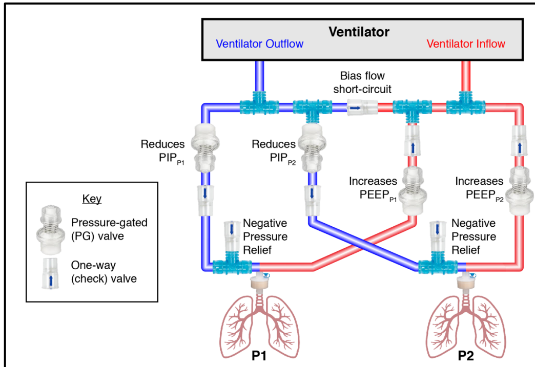
Figure 2: Schematic of PReVentS Ventilator Splitting design. Locations of modified in-line pressure-gated valves, and also one-way check valves to minimize cross-patient ventilation and allow individualized pressure controls, are shown. Functional impact of adjusting each pressure-gated valve is also indicated, for each patient.
