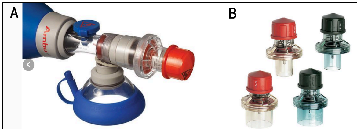
Figure 3: Photographs of single-use Ambu PEEP valves. (A) attached to a bag valve mask assembly; (B) individual PEEP valves that can be used in the PReVentS circuit. (from: https://www.ambuusa.com/products/airway-management/resuscitators/product/peep-valves ).
