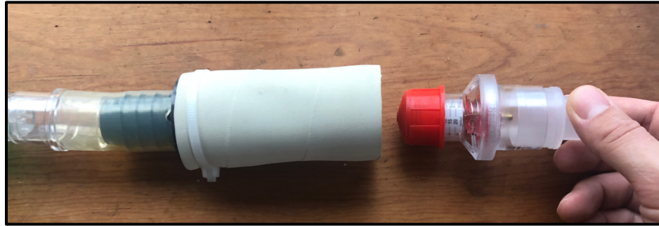
Figure 5: Final step of insertion of PEEP valve into flexible 1-5/8" tubing to produce the in-line PEEP valve for the PReVentS circuit.
