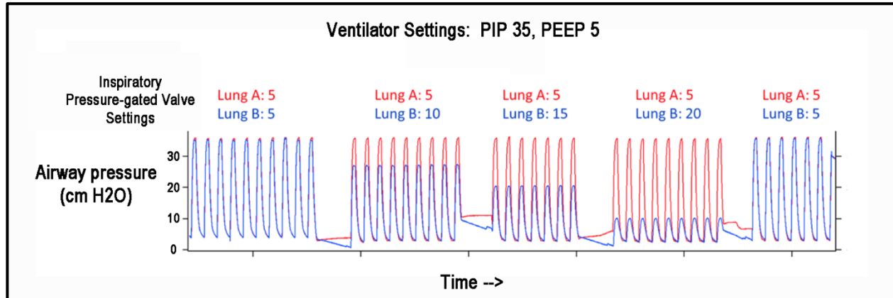
Figure 10: Impact of pressure-gated valve settings in inspiratory limb on ventilation pressures for two “patients”. Patient #1 corresponds to Lung A, while Patient #2 corresponds to Lung B. Inspiratory valve pressure settings are in cmH 2 O.
