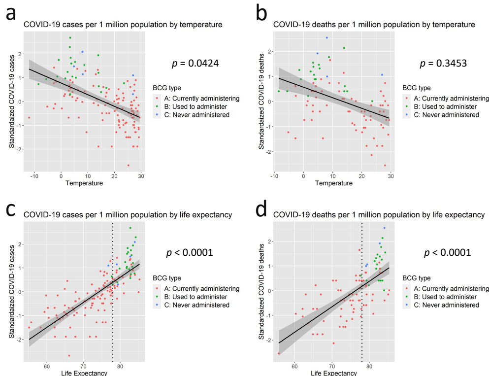
Figure 1: Correlations between temperature or life expectancy and COVID-19
