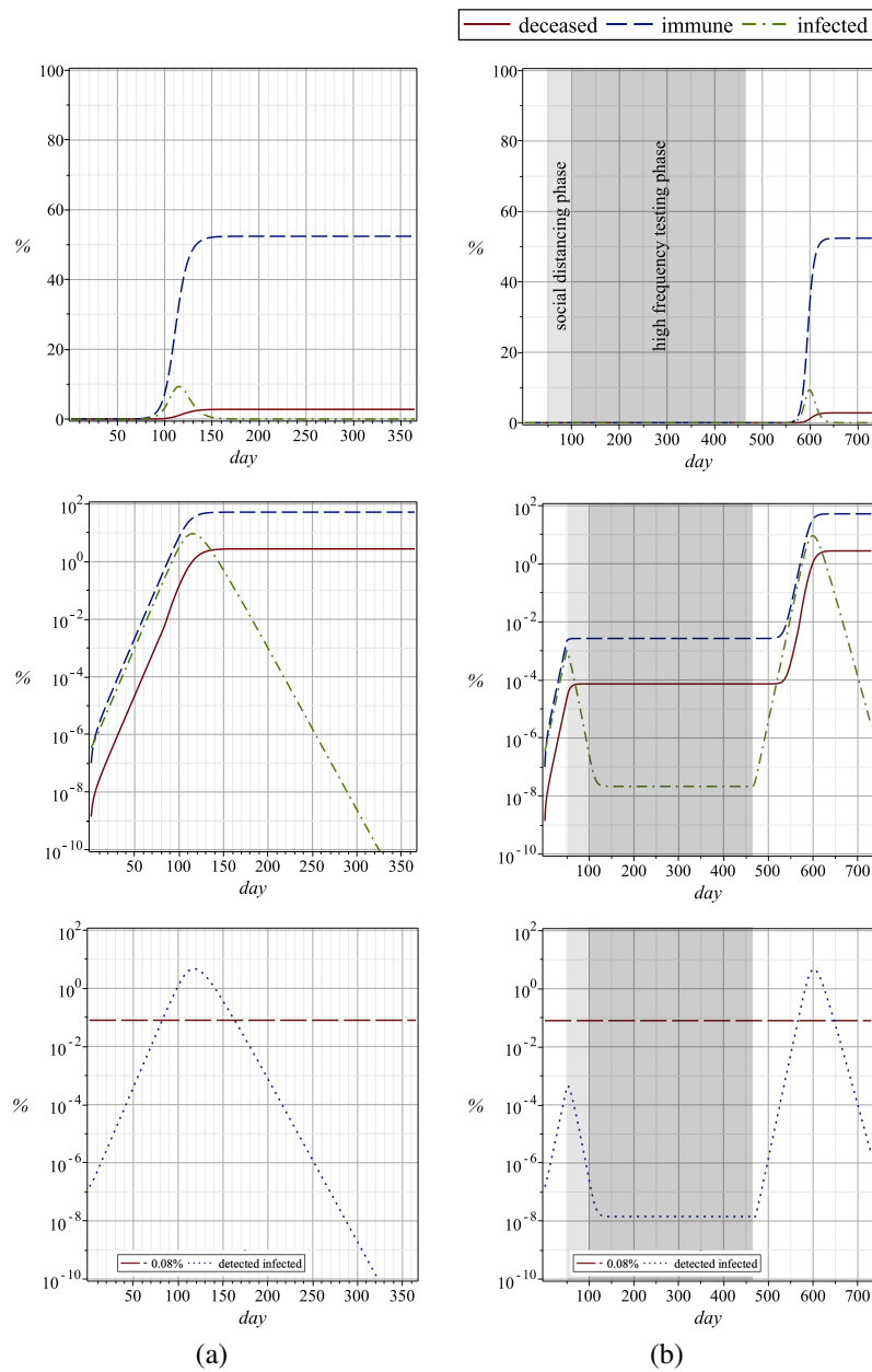
Figure 7: Combined strategy study. (a): base case (b): social distancing phase with 70% lower infection rate (50 to 100 days) followed by one year of high frequency testing with a 1.7666 times higher detection rate. Dashed lines represent the immune ( n_{s,init} - n_s(t) ), dash-dotted lines the infected ( n_{i_{lu}} + n_{i_{ld}} ) and solid lines the deceased ( n_k ) population; on the top with linear and in the middle with logarithmic scaling. In the bottom logarithmic plots the detected infected population (dotted lines) is shown together with the intensive care unit capacity (horizontal long dashed lines). The values are in % of the initial susceptible population size and are plotted over number of days. The light and dark gray shadings marks the "social distancing" and "more frequent testing" phases, respectively.
