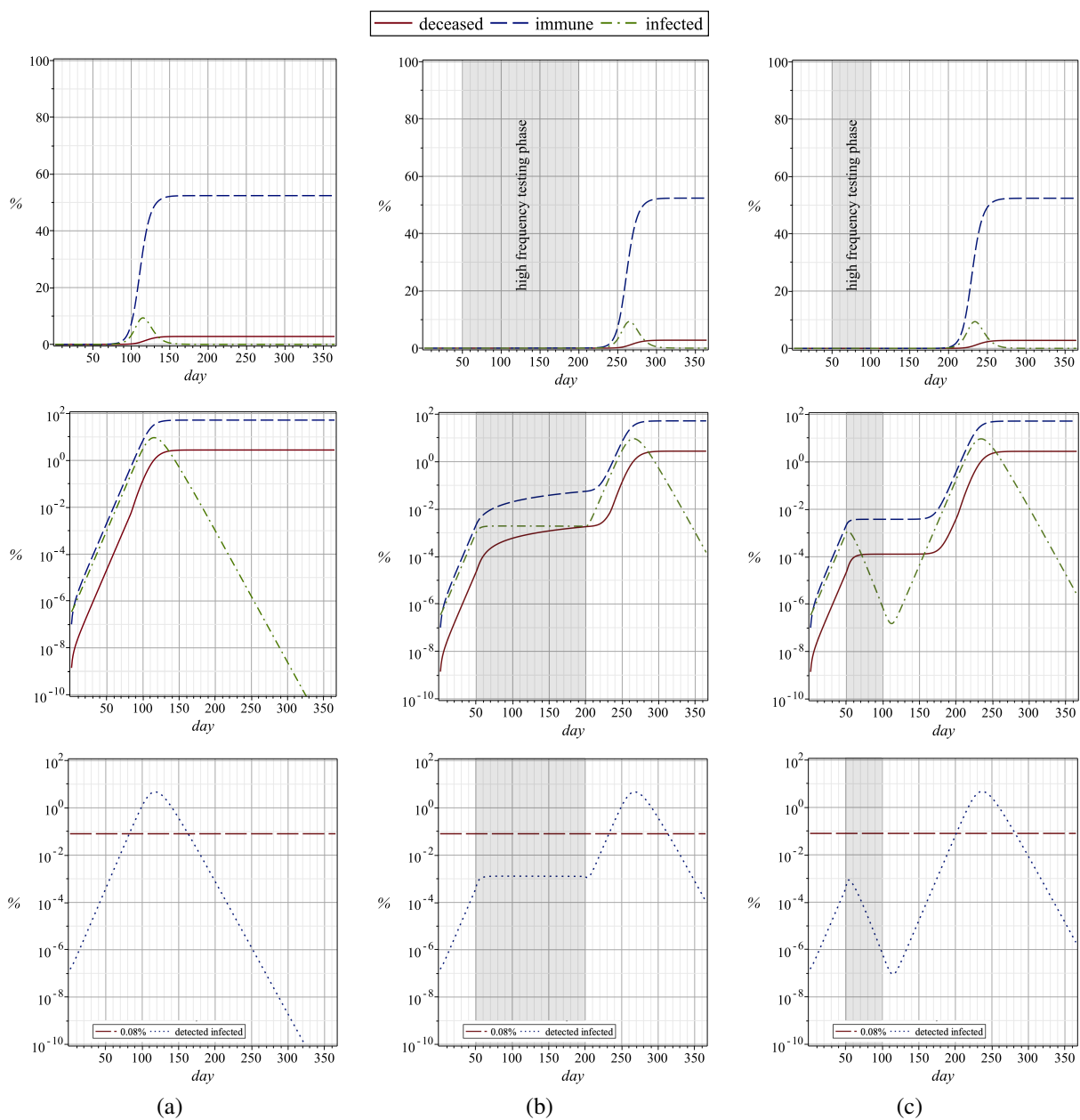
Figure 6: High frequency testing strategy studies. (a): base case (b): 1.7666 times higher detection rate (corresponding to a reproduction factor of one) in the period from 50 to 200 days. (c): 2.8240 times higher detection rate (same reproduction number as with 70% lower infection rate; see Fig. 5) in the period from 50 to 100 days. Dashed lines represent the immune ( n_{s,init} - n_s(t) ), dash-dotted lines the infected ( n_{fil} + n_{fid} ) and solid lines the deceased ( n_k ) population; on the top with linear and in the middle with logarithmic scaling. In the bottom logarithmic plots the detected infected population (dotted lines) is shown together with the intensive care unit capacity (horizontal long dashed lines). The values are in % of the susceptible population size and are plotted over number of days. The gray shading marks the "more frequent testing" phases.
