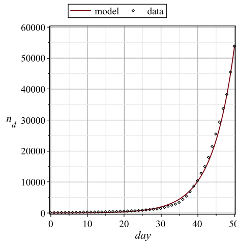
Figure 2: Model calibration: number of detected persons ( n_{i|d} + n_k + n_{r|d} ) computed by the model (line) compared with the data (circles) for the first 51 days.
