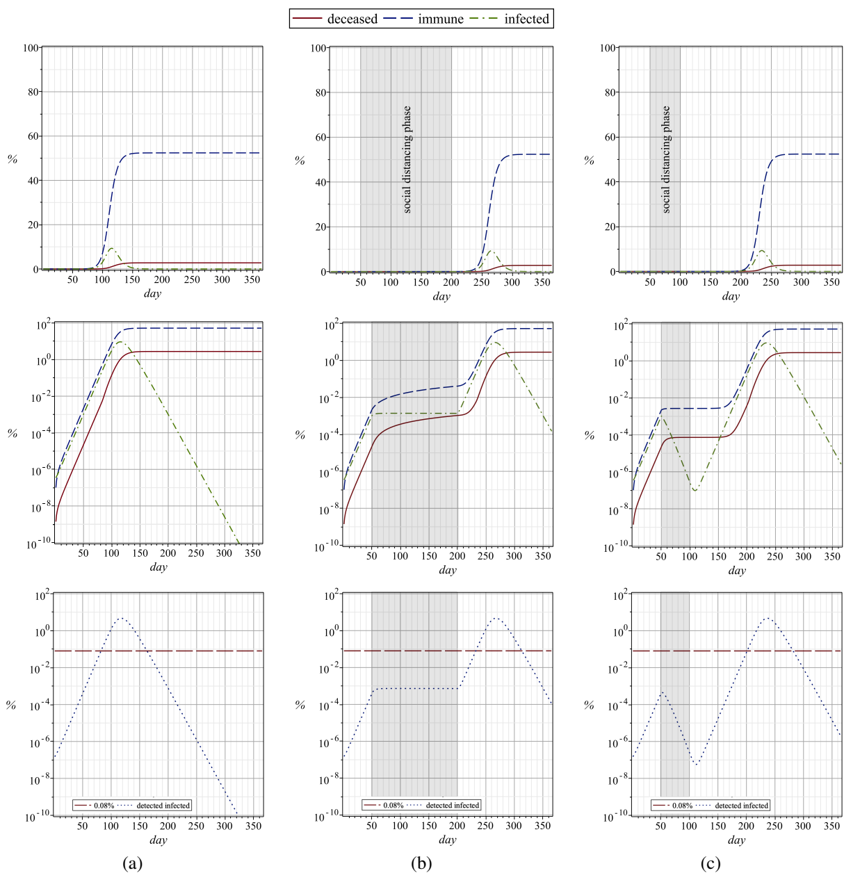
Figure 5: Social distancing strategy studies. (a): base case (b): 29.42% lower infection rate (corresponding to a reproduction factor of one) in the period from 50 to 200 days. (c): 70% lower infection rate in the period from 50 to 100 days. Dashed lines represent the immune ( n_{s,init} - n_s(t) ), dash-dotted lines the infected ( n_{ill} + n_{fid} ) and solid lines the deceased ( n_k ) population; on the top with linear and in the middle with logarithmic scaling. In the bottom logarithmic plots the detected infected population (dotted lines) is shown together with the intensive care unit capacity (horizontal long dashed lines). The values are in % of the initial susceptible population size and are plotted over number of days. The gray shading marks the "social distancing" phases.
