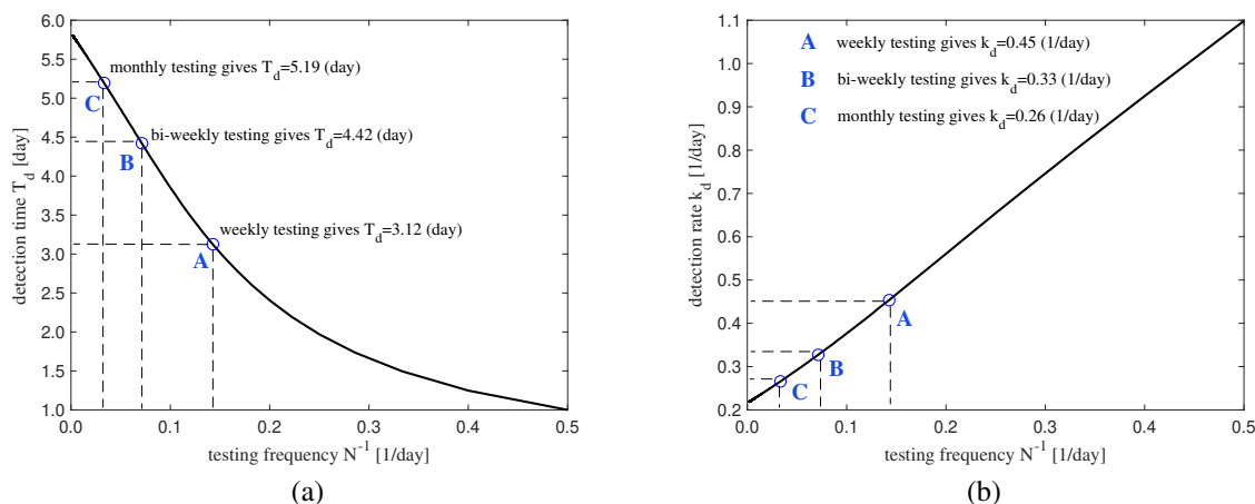
Figure 8: Average detection time and detection rate versus testing frequency. Note that the testing scenarios A, B and C are equivalent to testing random fractions of 1/7, 1/14 and 1/30, respectively, of the entire susceptible population every day.
