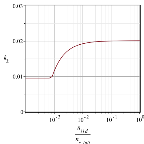
Figure 3: Effect of exceeding the capacity of the health care system on death rate. Average value of mortality rate k_k (probability per day for a detected infected person do die) as a function of the fraction \bar{n}_{i|d} of detected infected persons.
