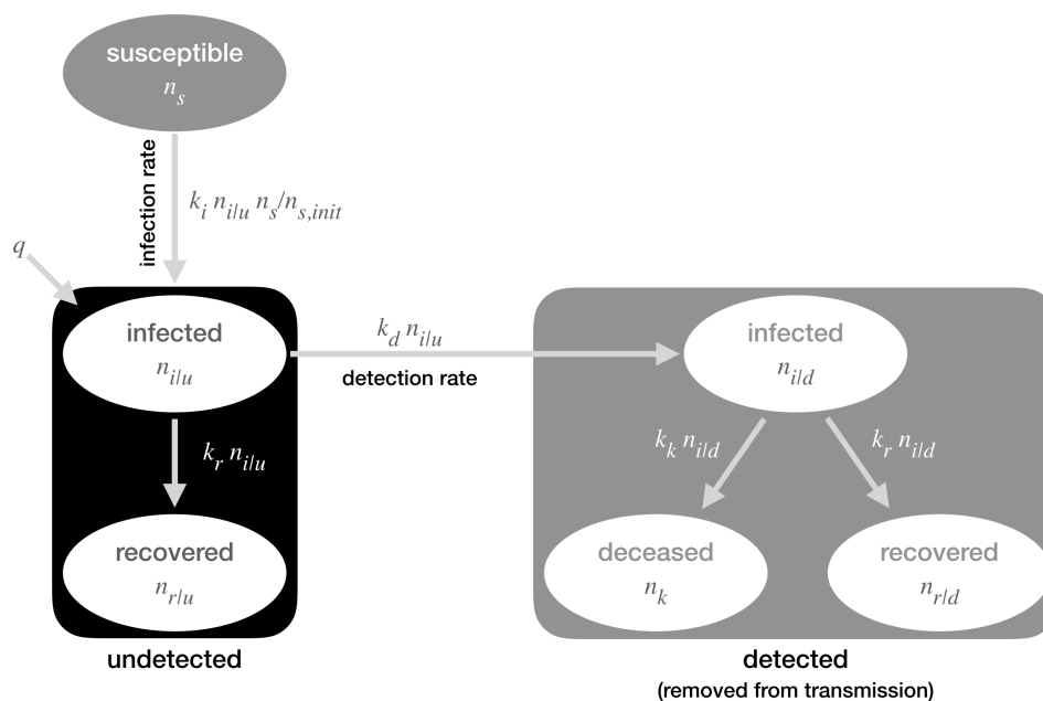
Figure 1: Graph showing the dependencies of the dynamic system describing the evolution of the numbers of undetected and detected infected persons ( n_{ilu} and n_{id} , respectively), the numbers of undetected and detected recovered persons ( n_{rlu} and n_{rld} , respectively) and the number of fatalities ( n_k ).
