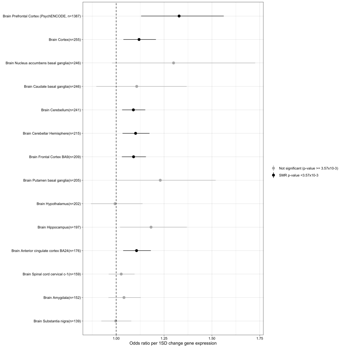
Figure 3. MR analysis of ACE expression in brain tissue with risk of schizophrenia. Forest plot of the effect of a 1 standard deviation (SD) decrease in ACE gene expression on schizophrenia risk in different brain regions. eQTL data was queried for 13 different brain regions from GTEX v8 and the prefrontal cortex region from PsychENCODE. Associations that are statistically significant after correcting for 14 tests ( p\text{-value} < 3.57 \times 10^{-3} ) are shown in black. The sample size (n) for each dataset is provided in brackets.
