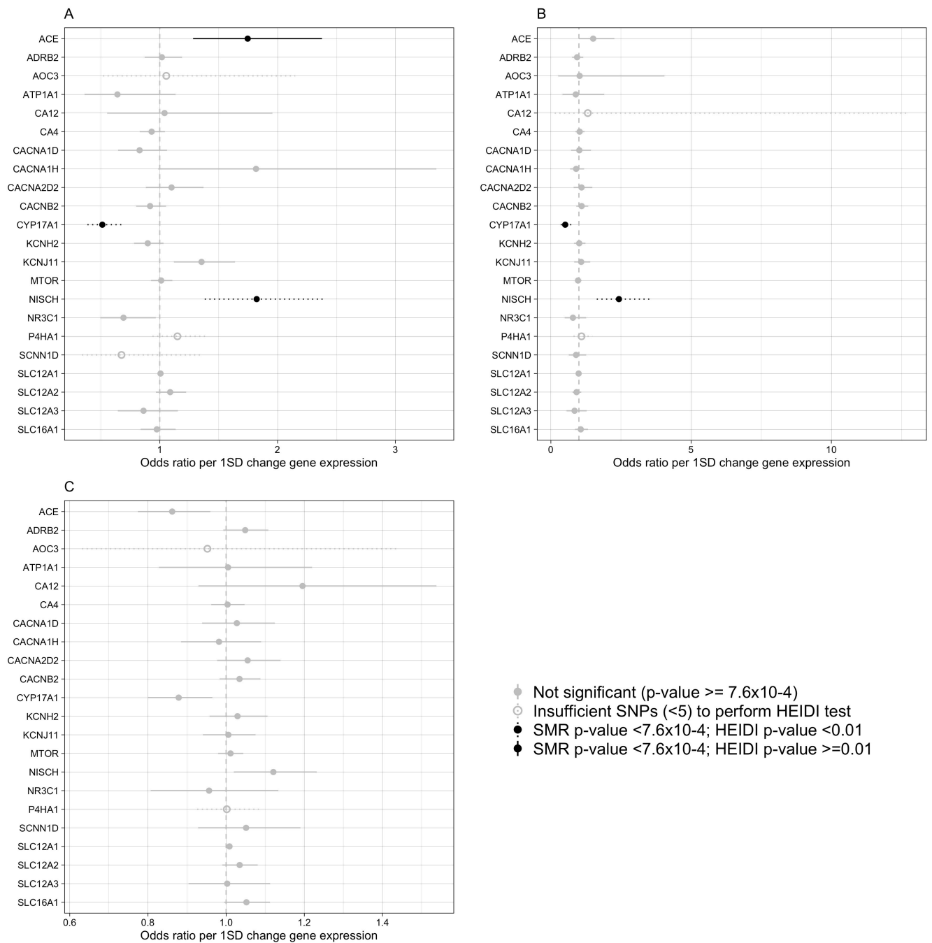
Figure 2. Association of drug target gene expression in blood with disease risk. Forest plot of the effect of a standard deviation (SD) change in expression of 22 BP-lowering drug target genes in blood on A) schizophrenia B) bipolar disorder C) major depressive disorder risk (odds ratio). Bars represent 95% confidence intervals. The direction of gene expression change reflects the SBP-lowering effect. An odds ratio > 1 suggests an increased risk of disease associated with the direction of gene expression change that is also associated lowering of blood pressure. Associations that are statistically significant after correcting for multiple testing (22 genes x 3 phenotypes; p -value < 7.6 \times 10^{-4} ) and that have a HEIDI p -value \geq 0.01 are shown by black lines. Associations that are statistically significant after correcting for multiple testing but have a HEIDI p -value < 0.01 (indicating association likely due to linkage) are shown in black dotted lines. Associations that did not pass the multiple testing correction are shown in grey lines. Associations for which a HEIDI test could not be performed due to unavailability of sufficient number SNPs (<5) are shown by grey dashed line.
