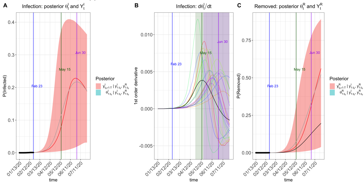
Figure 9: Prediction plots of \theta_t^I and Y_t^I (Panel A), \dot{\theta}_t^I (Panel B), \theta_t^R and Y_t^R (Panel C) for Hubei without intervention, \pi(t) \equiv 1 .
