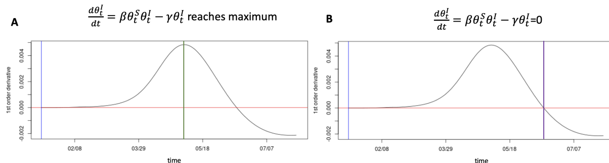
Figure 7: The first turning point in Panel A is marked by a green line, denoting the time when the estimated first-order derivative of the prevalence of infection reaches the maximum. The second turning point in Panel B is marked by a purple line, which is the time when the estimated first-order derivative of the prevalence of infection equals to zero. The vertical blue line labels the first observation day.
