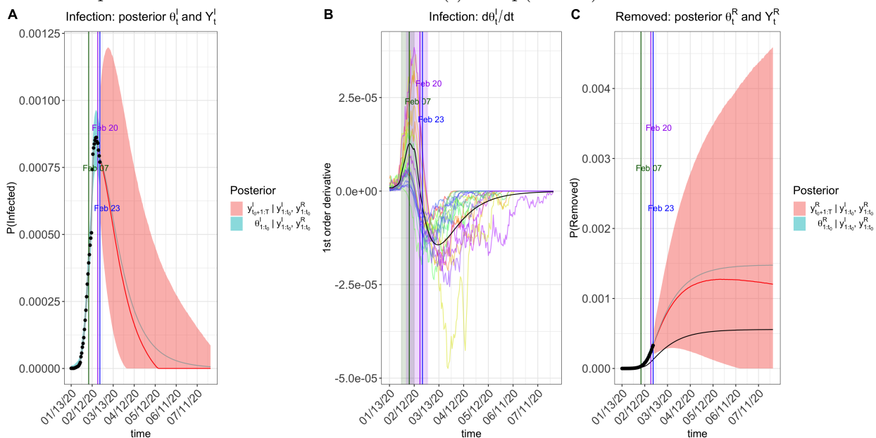
Figure 10: Prediction plots of \theta_t^I and Y_t^I (Panel A), \dot{\theta}_t^I (Panel B), \theta_t^R and Y_t^R (Panel C) for Hubei with an exponential transmission rate modifier \pi(t) = \exp(-0.05t) .
