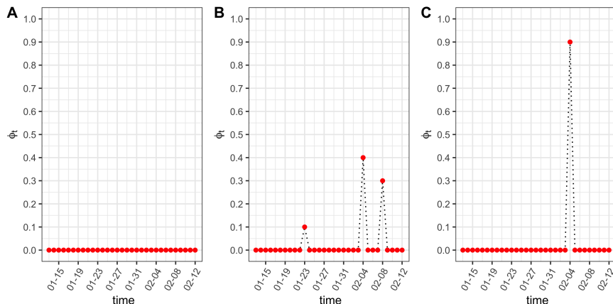
Figure 6: Three examples of multi-point instantaneous quarantine rates. Subfigures from A to C denote \phi_0 = (0, 0, 0, 0) , \phi_0 = (0.1, 0.4, 0.3) and \phi_0 = (0, 0.9, 0) at three time points of (Jan 23, Feb 4, Feb 8) respectively.
