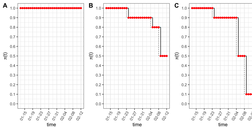
Figure 3: Transmission rate modifier takes different forms of step functions under different macro quarantine measures over time. Subfigures from A to C indicate \pi_0 = (\pi_{01}, \pi_{02}, \pi_{03}, \pi_{04}) equal to (1, 1, 1, 1) , (1, 0.9, 0.8, 0.5) and (1, 0.9, 0.5, 0.1) with change time points at (Jan 23, Feb 4, Feb 8) respectively.
