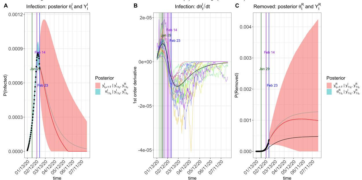
Figure 19: Prediction plots of \theta_t^I and Y_t^I (Panel A), \dot{\theta}_t^I (Panel B), \theta_t^R and Y_t^R (Panel C) for Hubei with an exponential transmission rate modifier \pi(t) = \exp(-0.05t) after data calibration.
