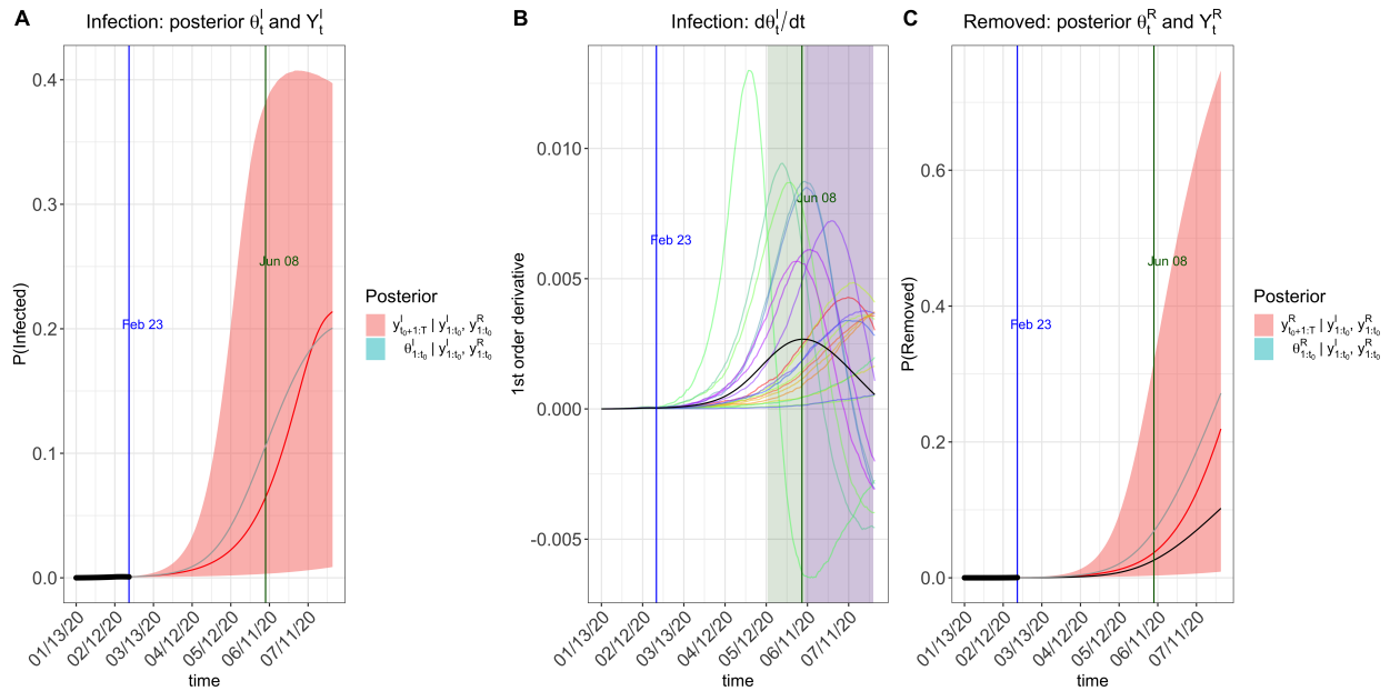
Figure 18: Prediction plots of \theta_t^I and Y_t^I (Panel A), \dot{\theta}_t^I (Panel B), \theta_t^R and Y_t^R (Panel C) for Hubei province with \pi(t) \equiv 1 after calibration. Note that the second turning point is beyond the time-axis limit in the plots.
