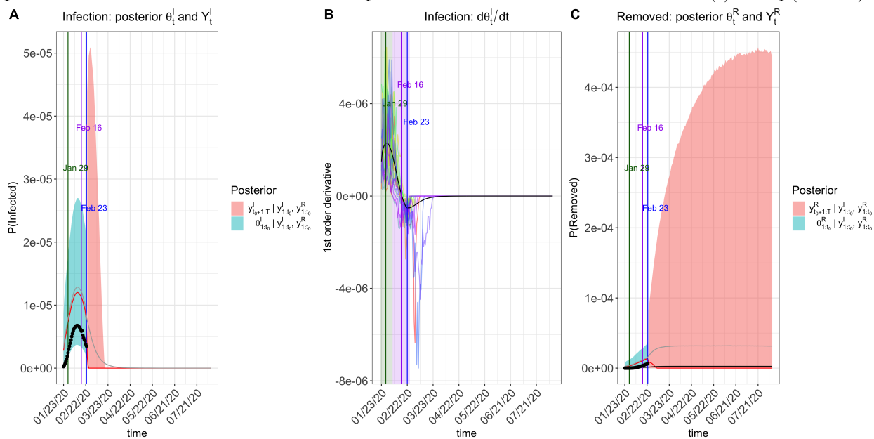
Figure 13: Prediction plots of \theta_t^I and Y_t^I (Panel A), \dot{\theta}_t^I (Panel B), \theta_t^R and Y_t^R (Panel C) for the other provinces outside Hubei with an exponential transmission rate modifier \pi(t) = \exp(-0.05t) .
