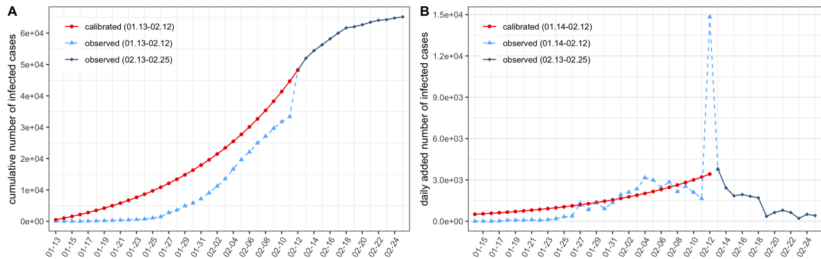
Figure 8: Under-reporting calibration of the infected cases in Hubei. (A) The cumulative number of infected cases. (B) The daily added number of infected cases. Data calibration is performed from Jan 13 to Feb 12 as is shown by the red curves.
