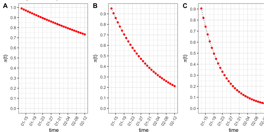
Figure 4: Transmission rate modifier takes continuous functions under difference micro quarantine measures over time. Subfigures from A to C are exponential survival functions with \lambda_0 = 0.01, \lambda_0 = 0.05 and \lambda_0 = 0.1 respectively.
