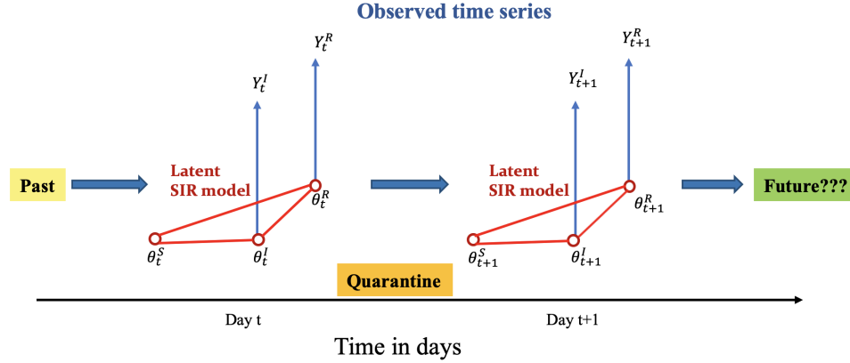
Figure 1: A conceptual framework of the proposed epidemiological state-space SIR model.
