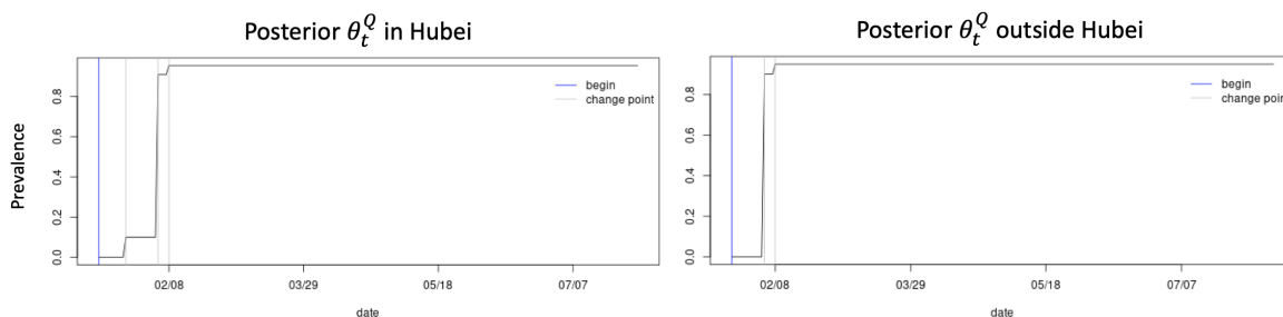
Figure 17: The posterior mean probability of staying in quarantine compartment within and outside Hubei.
