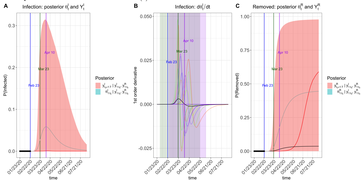
Figure 12: Prediction plots of \theta_t^I and Y_t^I (Panel A), \dot{\theta}_t^I (Panel B), \theta_t^R and Y_t^R (Panel C) for the other provinces outside Hubei with \pi(t) \equiv 1 .
