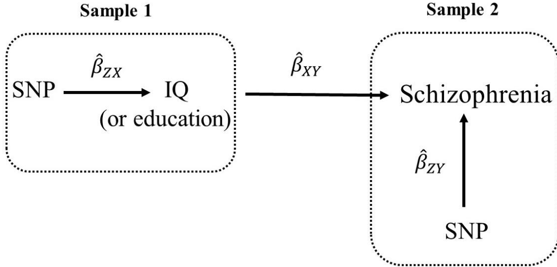
Fig. 5. Two-sample Mendelian randomization testing the causal effect of intelligence or education on schizophrenia. Estimates of the SNP-intelligence (or SNP-education) associations ( \hat{\beta}_{ZX} ) are calculated in sample 1 (from GWA study of intelligence or GWA study of education). The association between these same SNPs and schizophrenia are then estimated in sample 2 ( \hat{\beta}_{ZY} ) (from a schizophrenia GWA study). These estimates are combined into Wald ratios ( \hat{\beta}_{XY} = \hat{\beta}_{ZY} / \hat{\beta}_{ZX} ). The \hat{\beta}_{XY} estimates are meta-analyzed using the inverse-variance weighted analysis ( \hat{\beta}_{IVW} ) method. The IVW method produces an overall causal estimate of intelligence and/or education on schizophrenia.
