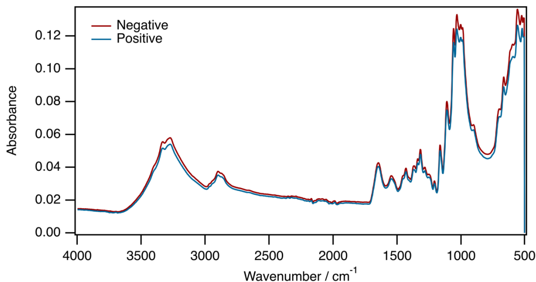
Fig. 3. Averaged mid-infrared spectra obtained from dried blood spots confirmed by PCR as Plasmodium positive or Plasmodium negative. Assignations of biochemical properties of different wavelengths are shown in Table 1.
