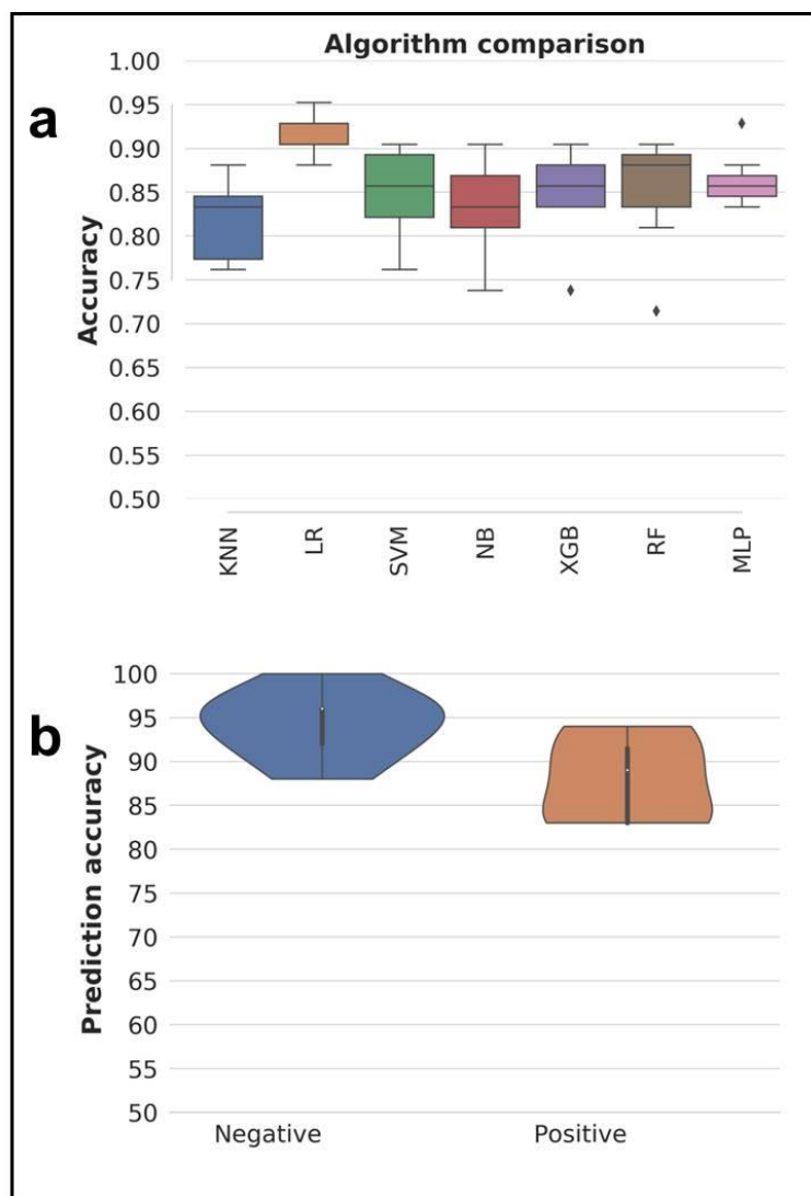
Fig. 4: (a) Prediction accuracies and precision for different classification models, based on PCR test results as reference. Models compared included k-nearest neighbors (KNN), logistic regression (LR), support vector machines (SVM), naïve Bayes (NB), XGBoost (XGB), random forest (RF), Multilayer perceptron (MLP). Logistic regression (LR) was the best performing model; (b) distribution of per class accuracies obtained by final LR classifiers and standard deviation from 70 bootstrapped models in predicting PCR test results from MIR spectral data.
