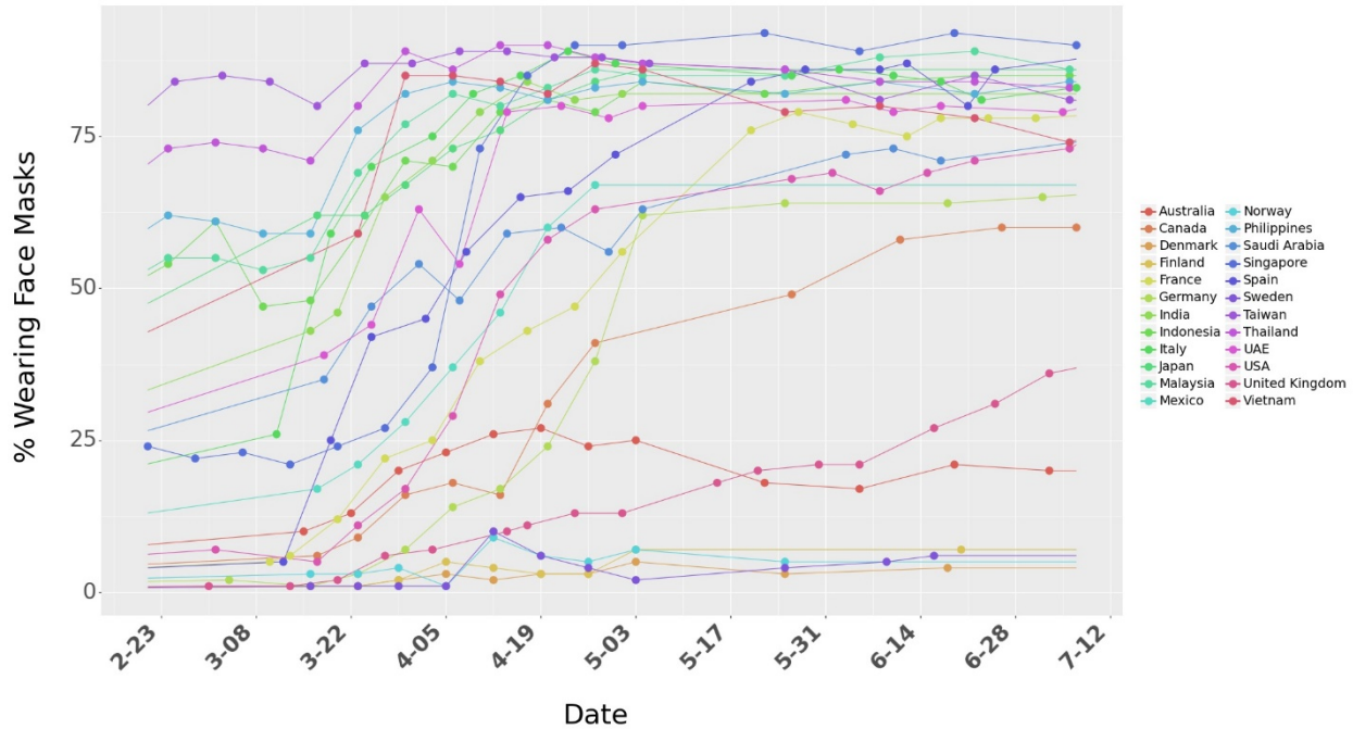
Figure 1. Percentage of people who say they are wearing a face mask in public spaces
