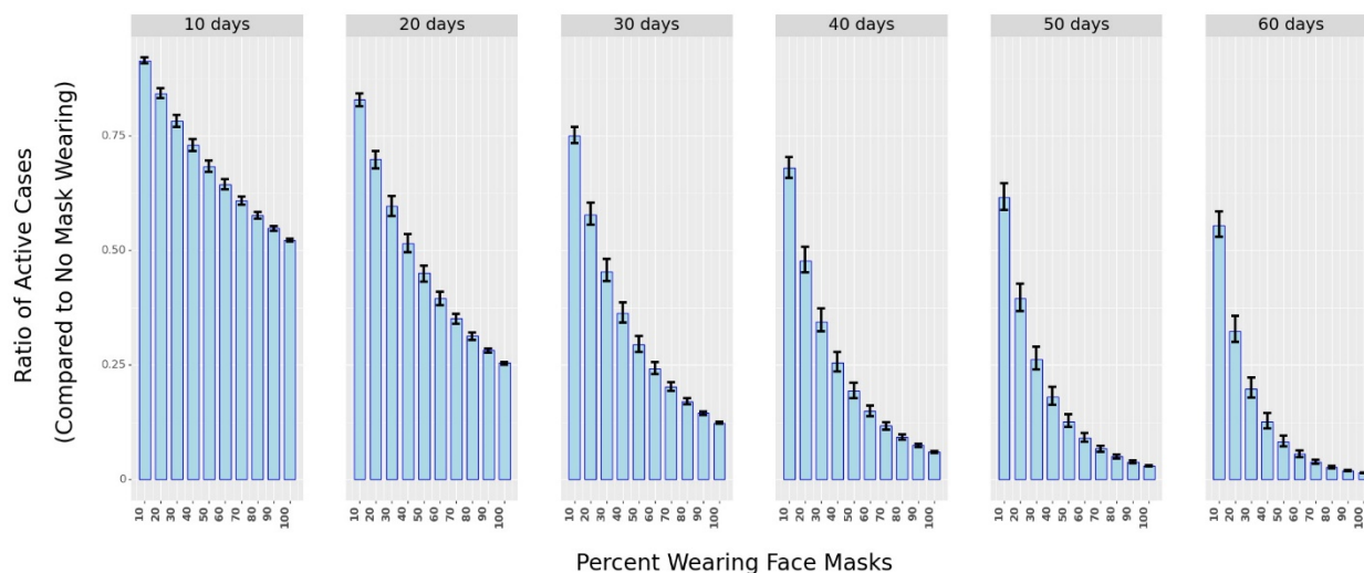
Figure 6. The ratio of Active cases under different percentages of mask-wearing in public spaces as compared to 0% mask-wearing over different periods (in days). The shaded bars represent in ratio while the black vertical lines represent the 25 th and 75 th percentile of the ratio (from simulations using Krinsky-Robb method)
