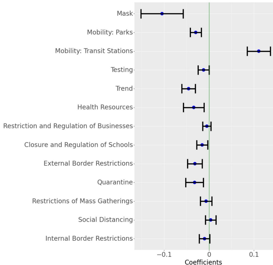
Figure 5. Parameter estimates for the Growth rate model. The blue dot indicates the point estimates and the horizontal lines indicate 95% confidence interval around the estimate (Masks transformed as \ln(1+\text{mask}) ). Results for different transformations of Mask and other covariates are shown in Figure S16.
