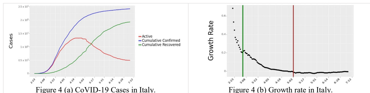
Figure 4. Daily Active cases and growth rate in Active cases for Italy. The vertical green line in (b) shows the start of data collection for Italy. The vertical red line in (b) shows the end of 60 days of data collection for Italy. Data for all 24 countries are shown in Figure S6 and Figure S7 respectively in the Supplement.
