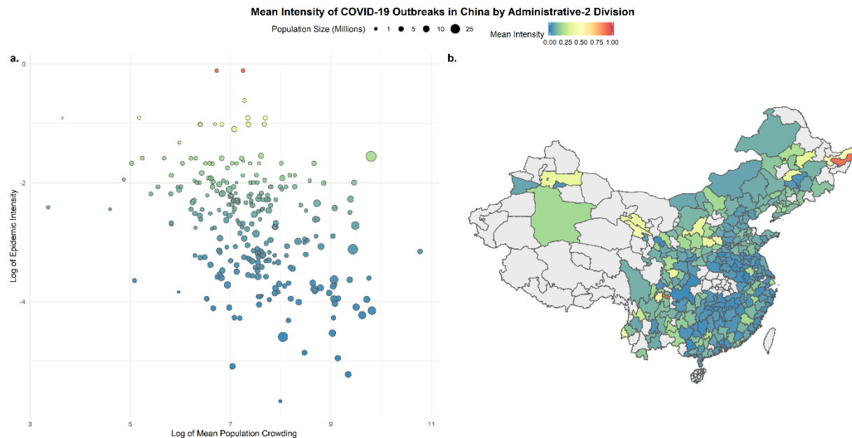
110 111 Figure 2: Crowding and the intensity of transmission of COVID-19 in China. a) negative association 112 between log of epidemic intensity, as measured by inverse Shannon entropy (Methods), and log 113 population crowding, as measure by Lloyd's mean crowding (Methods). Lower intensity and therefore 114 prolonged epidemics in larger cities. The size of the points indicate the size of the population in each city, 115 b) Map of epidemic intensity in China at the prefecture level. Darker colours indicate lower intensity and 116 lighter colours higher intensity. Grey prefectures had not enough reported cases, no cases or were not 117 included in analyses (Hubei Province).
