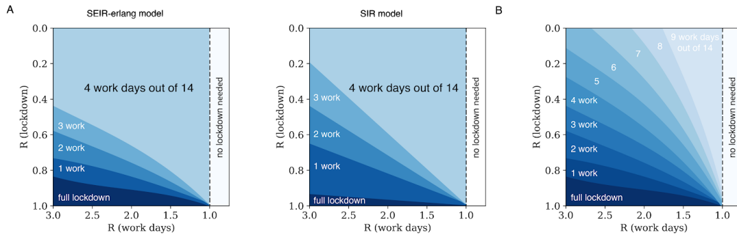
Fig. S3 A SIR deterministic model captures some of the effects. (A) The SIR model (right panel) lacks the exposed (non-infectious) compartment. It shows that the cyclic lockdown strategies can control the epidemic, but at smaller parameter regions for each given strategy than the SEIR-Erlang model (left panel). The difference is biggest at large ratios of R at work and lockdown, where SEIR-Erlang has an advantage. The SIR model is dS/dt = -\beta SI , dI/dt = \beta SI - \gamma I . The replication number is R = \beta/\gamma . Here \gamma = 1/7 \text{ day}^{-1} (the plot is unaffected by this parameter), and S=1 . Effective R in the SIR model is the average R weighted by the fraction of time for work and lockdown. For analytical work on optimal epidemic control in the SIR model see [ https://osf.io/rq5ct/ ]. Note that the axes in this plot are inverted with respect to Fig 3. (B) In this figure, each region shows the maximal number of workdays where the epidemic can be suppressed for the SEIR erlang model, for work days in the range of 0-11.
