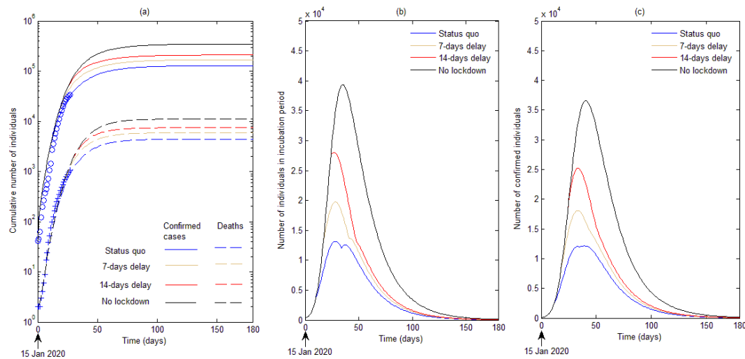
Figure 1. (a) Calibration of reported confirmed 2019-nCoV cases and deaths in Hubei province, China; (b) number of individuals in incubation period and (c) confirmed individuals over time for four scenarios: status quo (lockdown during 23 rd January to 12 th February 2020), 7-days delay, 14-days delay, and ‘no lockdown’.
