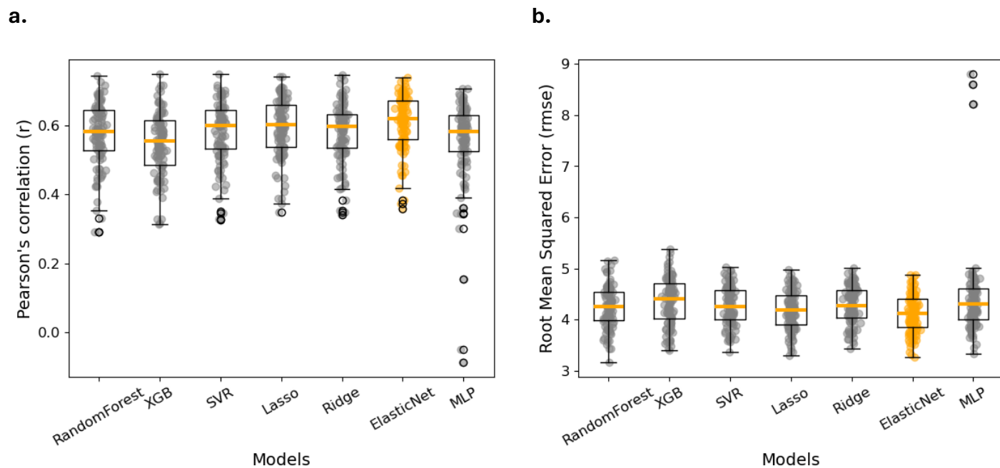
Figure 1. Model performance comparison. a) The distribution of the correlation coefficient ( r ) from the 100-fold cross validation. The Elastic Net Regression (orange) has the highest median r score ( r = 0.61 ), and b) the lowest mean RMSE (RMSE = 4.12).
