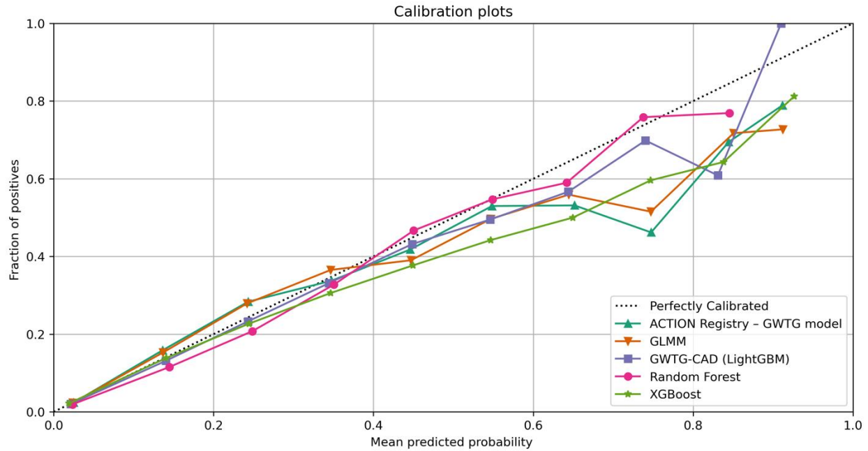
Figure 2. Calibration of prediction models using the held-out test set.
