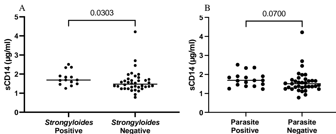
160 161 Figure 1. Soluble CD14 levels in those with and without parasites. Participants with 162 strongyloidiasis had higher sCD14 levels ( \mu\text{g/ml} ) compared to participants without 163 strongyloidiasis (1.69 vs. 1.48 \mu\text{g/ml} , respectively) (A). There was a higher sCD14 level ( \mu\text{g/ml} ) 164 in individuals with either positive Strongyloides serology or positive qPCR for parasites not 165 including Blastocystis (1.69 vs. 1.51 \mu\text{g/ml} , respectively) although not statistically significant 166 (B).
