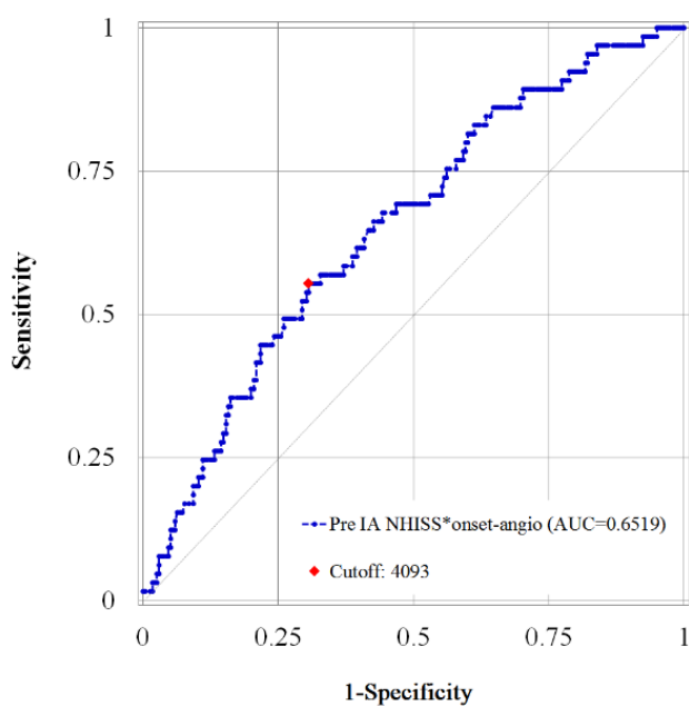
Figure 2. Receiver operating characteristic curve. The receiver operating characteristic (ROC) curve for pre-EVT NIHSS-time score and favorable neurological outcome. The Area under the curve is 0.6519. The best cut off pre-EVT NIHSS-time score value was 4093.
