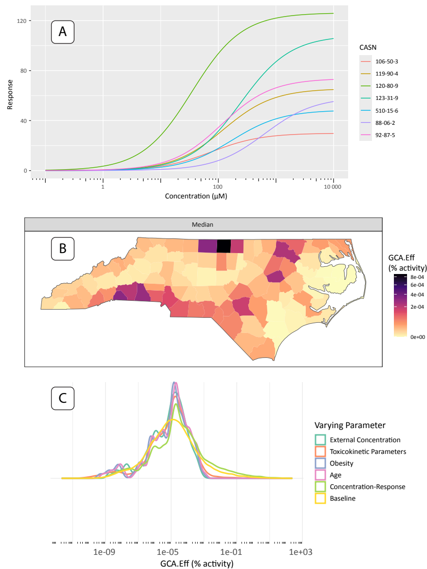
Fig. 4: Single assay results and plots produced by the GeoTox package. (A) Fitted dose-response plots for the 2-parameter hill model of the 7 chemicals with hit-calls on the H2AX histone modification genotoxicity assay. (B) Median generalized concentration addition (GCA) response or effect (GCA-Eff, units = percent activity) mapped to the county level. (C) Sensitivity analysis results shown as smoothed kernel densities by analysis parameter.
