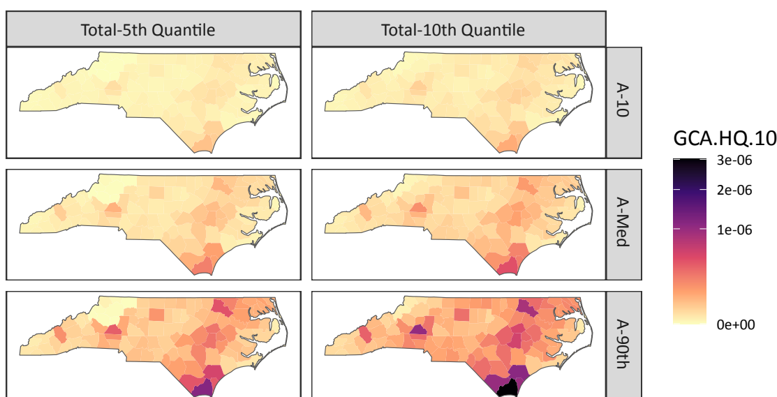
Fig. 5: Multi-assay risk summaries mapped across North Carolina counties using the GCA based hazard quotient. Rows are the individual assay level summarization of 10th, 50th, and 90th quantiles, respectively. The columns are the total summarization as the 5th and 10th quantile, respectively.
