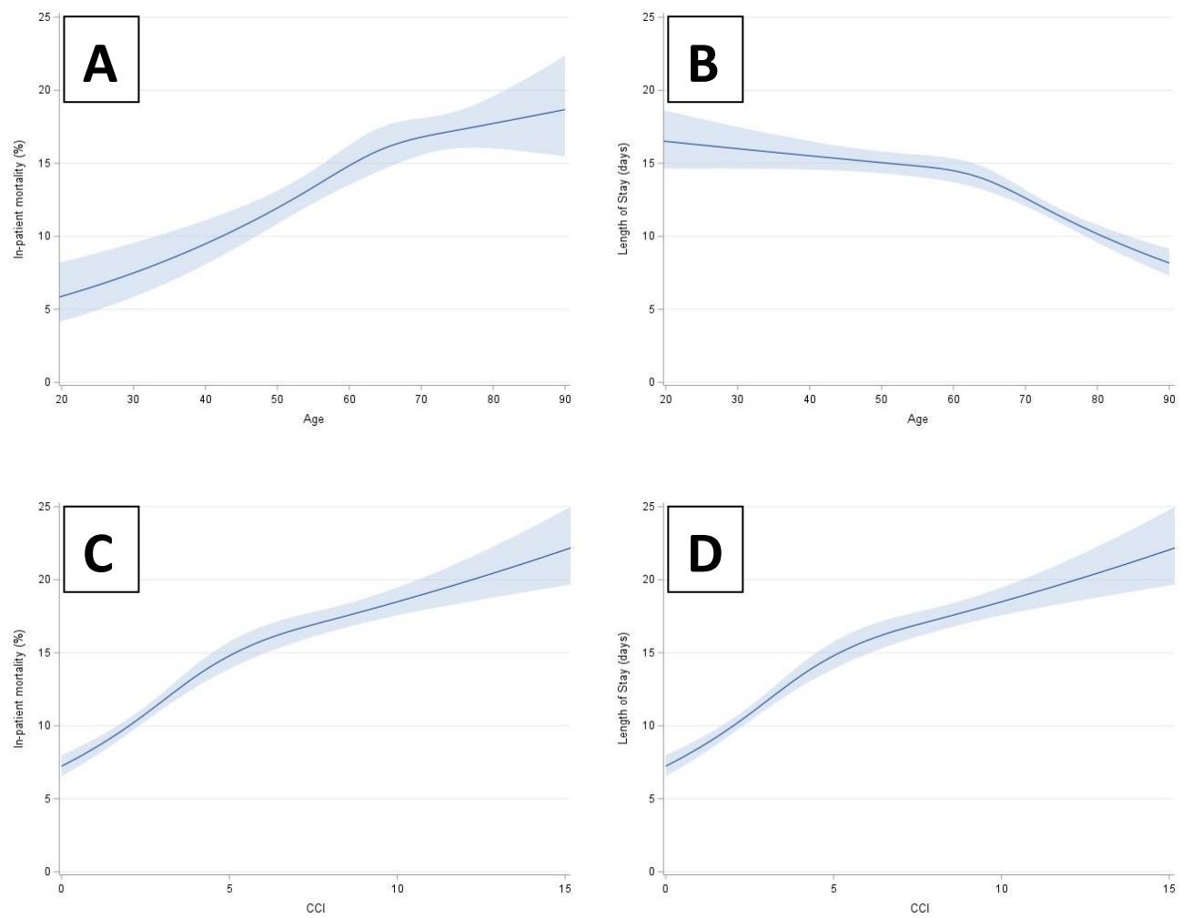
Figure 1. The effect of age (top row) and comorbidity burden (bottom row) on inpatient mortality (left column) and length of stay (right column) for hospitalizations of patients with a spinal cord infarction.
