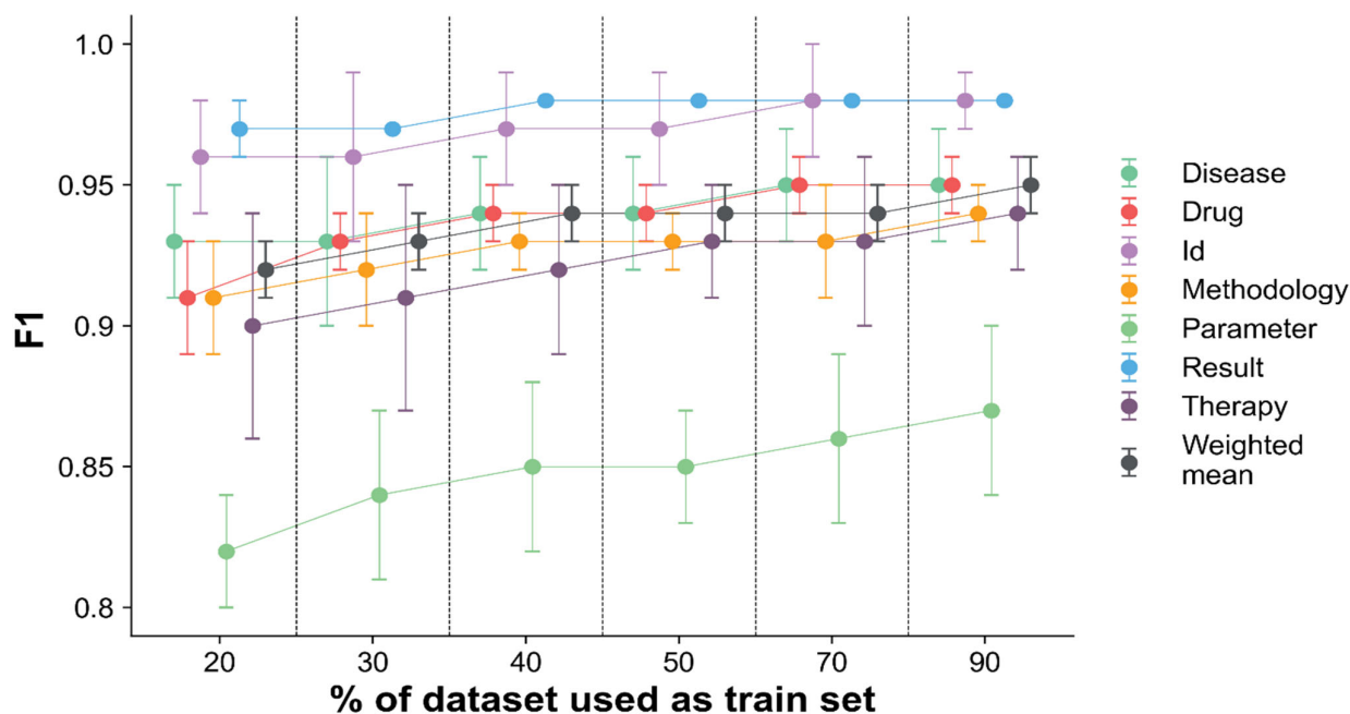
Figure 3 – Effect of limiting the volume of train data on the model quality. Weighted mean F1 does not dip below 0.9 even when 80 annotated abstracts are used for finetuning. Mean F1 steadily increases up to 0.95 with full use of train corpus (90% of the dataset). Individual label classes show a similar trend, with a relatively steep increase in context understanding for the Parameter label class, improving up to 0.05 in F1.
