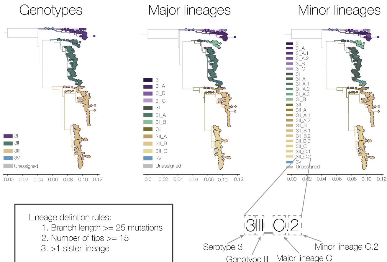
Figure 2 | Description of proposed dengue virus lineage classification system using serotype 3 as an example. Genotype level classification has been expanded to include most previously unassigned genomes. Two additional layers of classification have been proposed, major and minor lineages, the rules of which are shown here. The nomenclature is described here in its shorthand form (e.g. DENV-3III_C.2), with each element highlighted by a dotted box. The new lineage classifications for serotypes 1, 2, and 4 are shown in Figure S2 .
