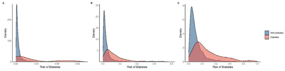
Figure 4. The distribution of the predictive probability of developing diabetes among participants with prediabetes by incident diabetes status within 1- year (A), 5-year (B), and 10-year (C).
