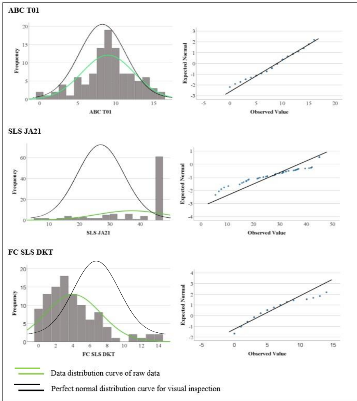
Figure 1. Graphical checking of the normal distribution using histograms and Q-Q plots for the total study population comparing competitiveness with established balance field tests
