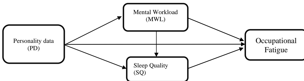
Figure 1. SEM conceptual framework
