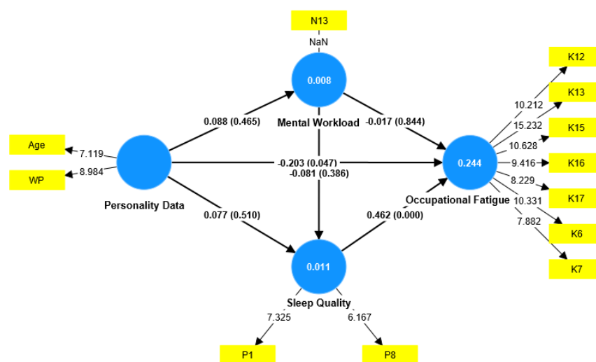
Figure 2. Conceptual Model SEM-PLS
