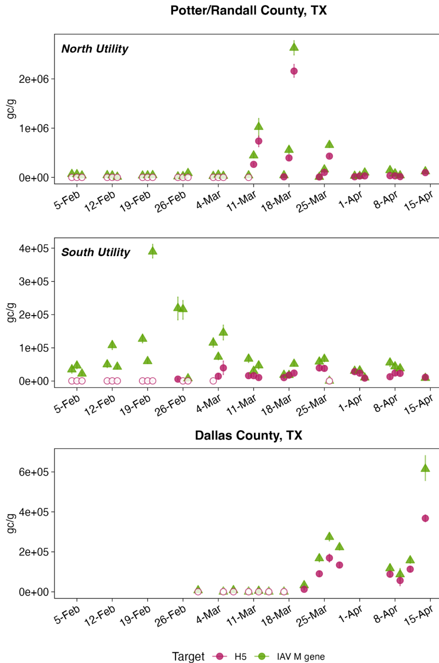
Figure 1. Concentrations of IAV M gene target (labeled as IAV, in green) as well as the H5 marker (labeled H5) and associated standard error in units of copies per gram dry weight; if error bars cannot be seen, then they are smaller than the symbols. Open markers are below the lowest measurable concentration (1000 copies per gram dry weight).
