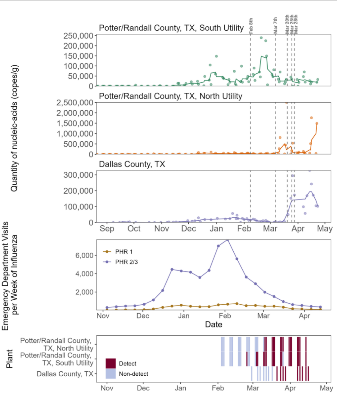
Figure 2. Top three panels. Concentrations of the IAV M gene in wastewater solids at the three WWTPs in Texas, as measured in the prospective monitoring. Line represents the 5-adjacent sample trimmed average, the symbols show the measured concentrations and the standard errors. Fourth panel from the top shows emergency department visits per week for influenza; PHR 1 represents Texas Public Health Region 1 (containing Potter/Randall Counties) and PHR2/3 represents Public Health Region 2/3 containing Dallas County. Bottom panel shows the presence or absence of the H5 marker in the samples from the three plants. Vertical lines indicate key dates as follows. February 8, 2024 USDA declares ongoing HPAI poultry outbreak, March 7, 2024: Unknown dairy cattle illness first reported, March 20, 2024: Samples collected from dairy cattle in Texas, March 25, 2024: Texas confirms H5N1 in dairy cattle, March 28, 2024: Positive H5N1 specimen collected from human.
