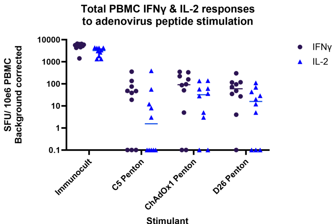
244 245 Figure 3 legend: Analysis of AdV specific IFN \gamma and IL2 FluoroSpot responses to AdV peptide pools (A) 246 IFN \gamma FluoroSpot responses to AdV peptide pools covering: the pentons of human adenoviruses C5 247 and D26, and the penton of chimpanzee adenovirus Y25 (vector backbone ChAdOx1) as well as a 248 polyclonal anti-CD3/CD28 antibody T cell stimulation as a positive control of PBMC from healthy 249 blood donors, calculated as spot-forming units (SFU) per 10e6 PBMC (background corrected). (B) IL2 250 FluoroSpot responses to AdV peptide pools covering: the pentons of human adenoviruses C5 and 251 D26, and the penton of chimpanzee adenovirus Y25 (vector backbone ChAdOx1) as well as a 252 polyclonal anti-CD3/CD28 antibody T cell stimulation as a positive control of PBMC from healthy 253 blood donors, calculated as spot-forming units (SFU) per 10 6 PBMC (background corrected).
