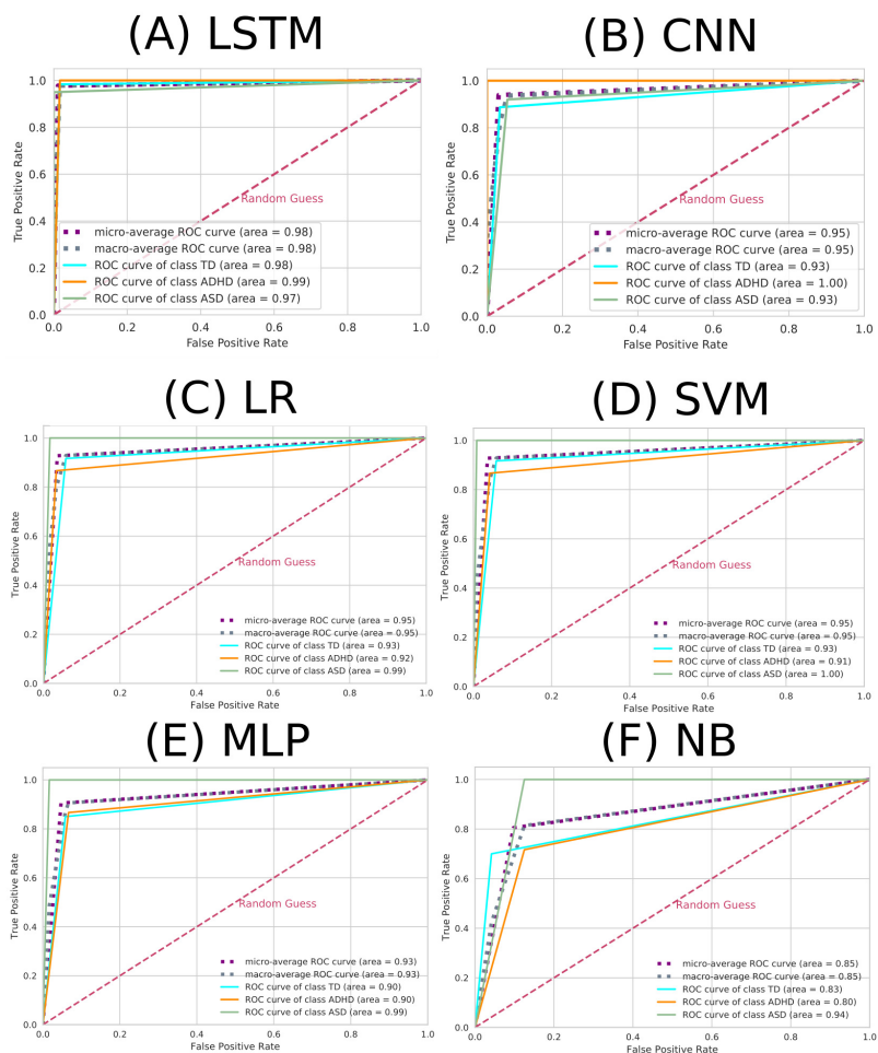
Fig 3. ROC curve for each ML algorithm. The elements in the figure labeled A to F correspond to LSTM, CNN, LR, SVM, MLP, and NB, respectively. The dashed pink line represents the random choice classifier, the purple line the micro-average ROC curve, the gray line the macro-average ROC curve, the turquoise line the ROC curve referring to the TD class, the orange line the ROC curve referring to the ADHD class, and the green line the ROC curve referring to the ASD class.
