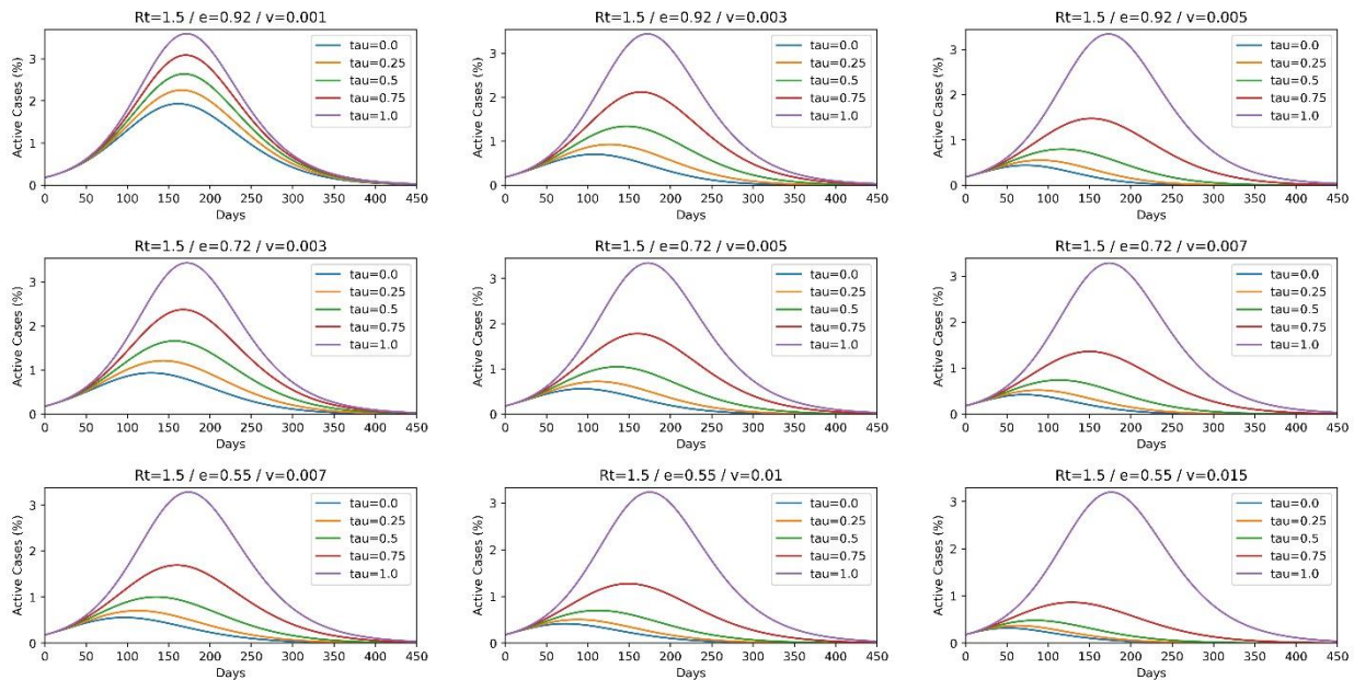
Figure 5. Graph showing the percentage of active cases in a population similar to that of Djibouti. The data collected was collected using the same initial conditions and vaccination schemes as Fig. (4).
