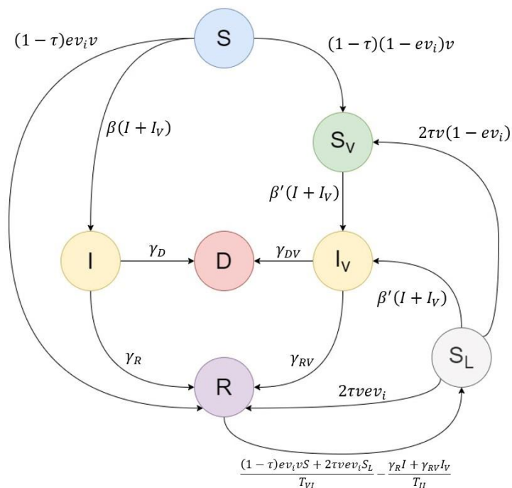
Figure 1. Schematic diagram showing the 7 compartments of the Booster model: Susceptible ( S ), Susceptible Vaccinated ( S v ), Susceptible with Lost immunity ( S L ), Infected ( I ), Infected Vaccinated ( I v ), Recovered ( R ), Dead ( D ) - along with the transfer dynamics between them.
