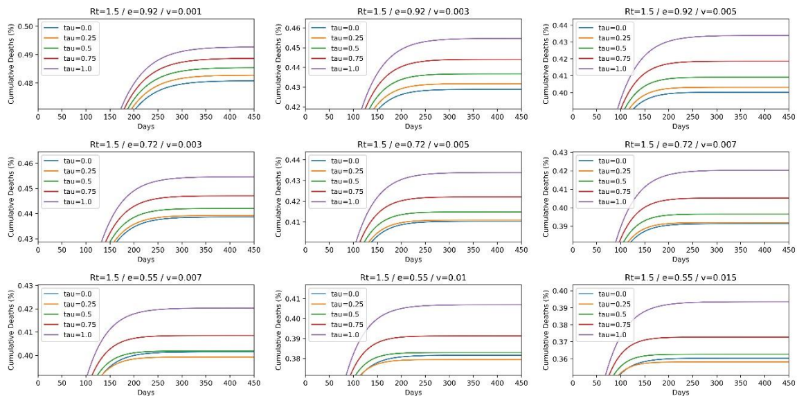
Figure 2. Graphs showing the percentage of cumulative deaths in a population with infection characteristics similar to those of Russia with a transmission coefficient of R=1.5 with initial conditions: 1.84% currently infected, 27.12% currently immune, 22.62% currently susceptible with lost immunity, 0.23% currently dead. Data collected using the following 9 vaccination schemes: e=92\% and v=0.1\% , e=92\% and v=0.3\% , e=92\% and v=0.5\% , e=72\% and v=0.3\% , e=72\% and v=0.5\% , e=72\% and v=0.7\% , e=55\% and v=0.7\% , e=55\% and v=1\% , e=55\% and v=1.5\% , with v_i = 90\% .
