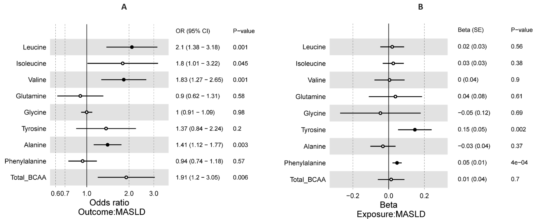
Figure 2 Forest p lots showing the effects of amino acids on MASLD (A) and MASLD on amino acids (B) using the inverse variance-weighted method. CI: Confidence interval. SE: Standard error. Solid dots indicate significance with p < 6.25 \times 10^{-3} . Hollow circles indicate non-significance with p \geq 6.25 \times 10^{-3} .
