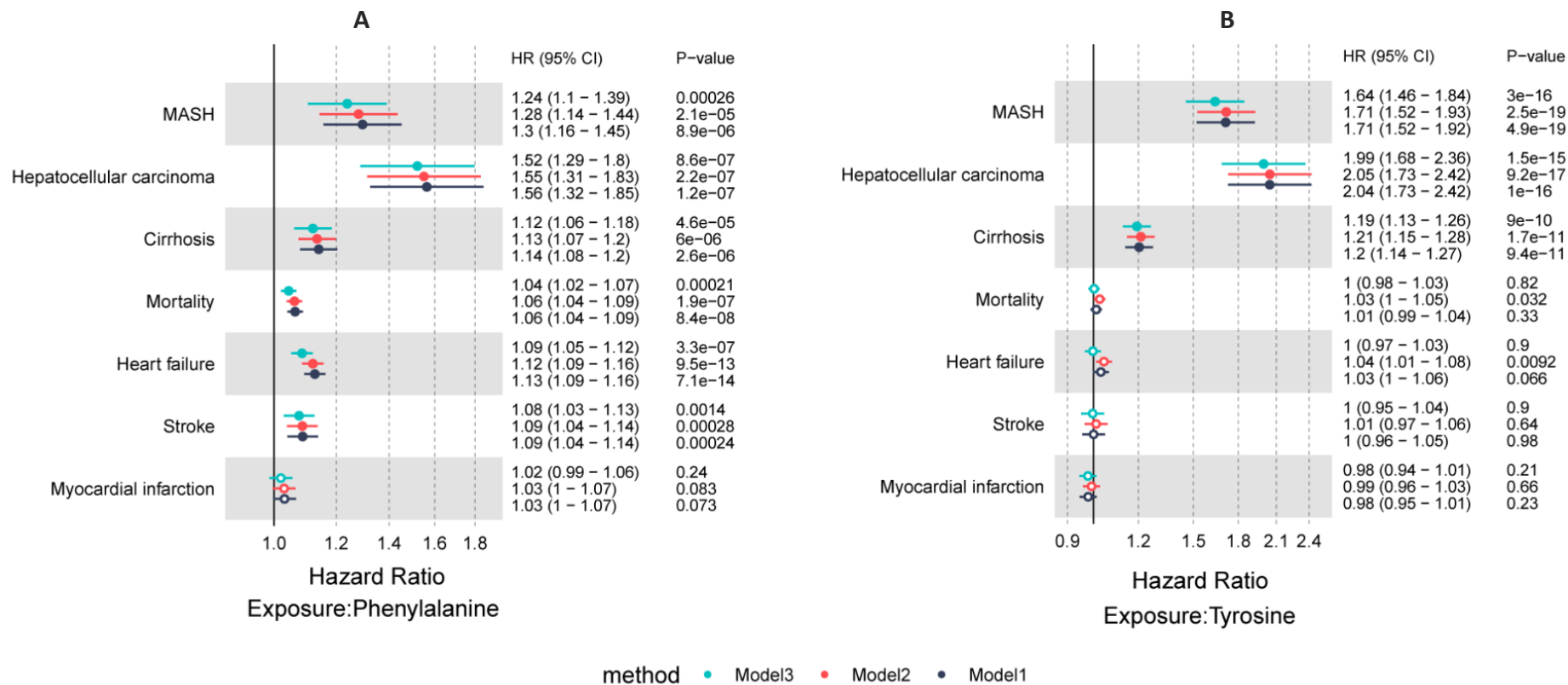
Figure 4 Forest plot showing the associations of phenylalanine (A) and tyrosine (B) with incidence of major outcomes in MASLD patients. CI: Confidence interval. Solid dots indicate significance with p < 7.1 \times 10^{-3} . Hollow circles indicate non-significance with p \geq 7.1 \times 10^{-3} .
