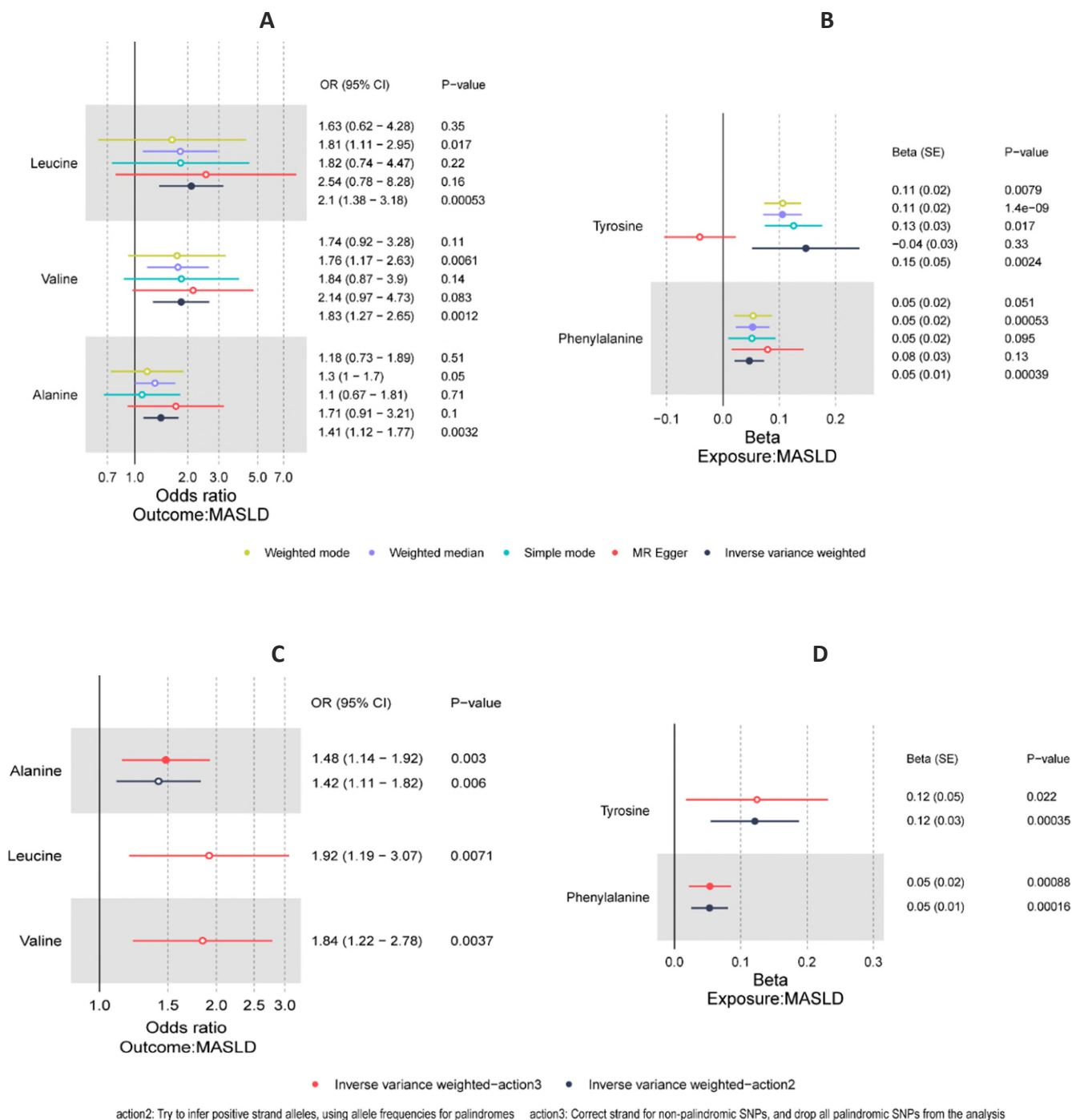
Figure 3 Forest plot showing the effects of leucine, valine, alanine on MASLD and MASLD on tyrosine and phenylalanine. (A-B) Using different Mendelian randomization analyses; (C-D) Using the inverse variance-weighted method with stricter conditions. CI: Confidence interval. SE: Standard error. Solid dots indicate significance with p < 6.25 \times 10^{-3} . Hollow circles indicate non-significance with p \geq 6.25 \times 10^{-3} .
