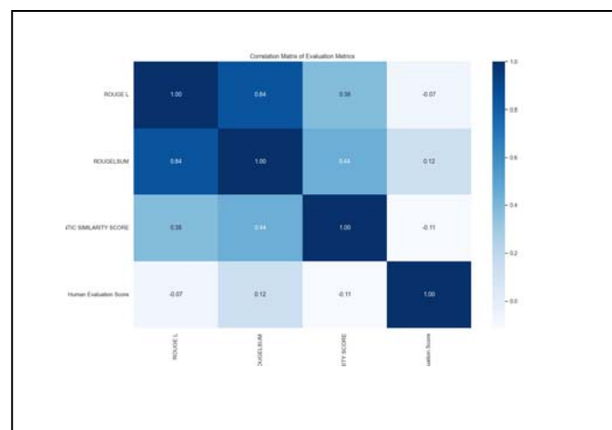
Fig. 3. Correlation between automated metrics and human evaluation
