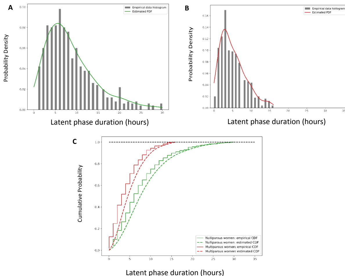
Figure 2: Empirical distributions and estimated distributions of the latent phase duration for nulliparas and multiparas, estimated from the data reported in Friedman. 8,9
