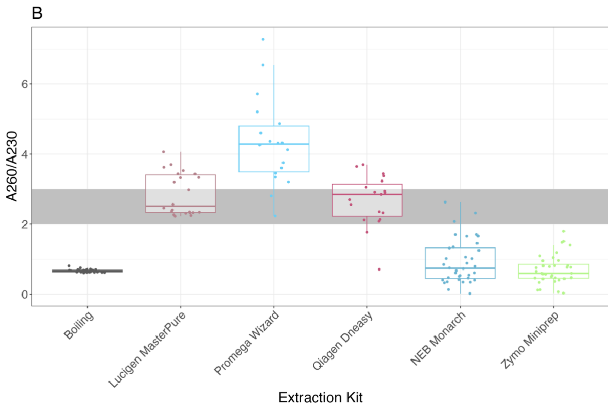
Figure 4 Absorbance ratios (A) A260/280 and (B) A260/230 indicating the presence of contamination and quality of DNA, respectively, of the extracted DNA extracted using six extraction methods. Technical (each sample extracted in
