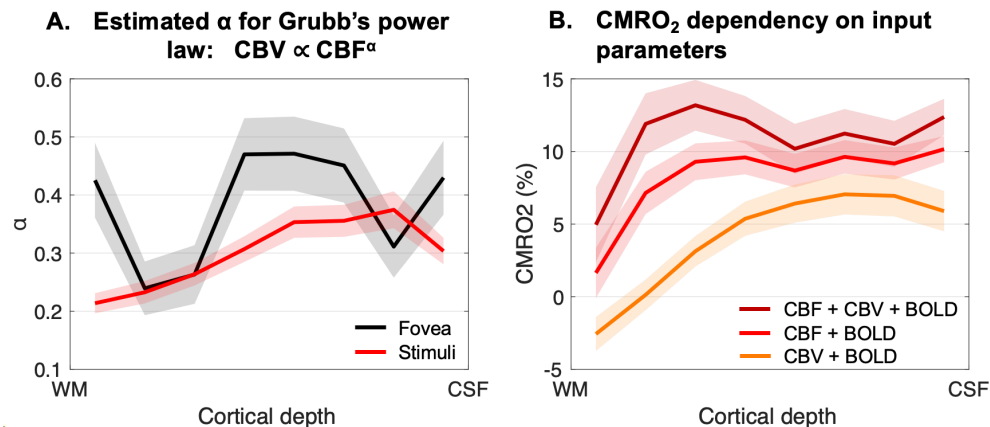
Supplemental Figure S4. A. Estimated \alpha values in the stimuli and fovea regions using CBF and CBV measurements. B. Comparisons between CMRO 2 measured from BOLD and simultaneously measured CBF and CBV (reference, dark red trace), or with only CBF (light red trace) or CBV (orange trace). When only CBF or CBV was used for CMRO 2 calculation, the Grubb's power law was utilized to generate the corresponding CBV or CBF respectively. Eccentricities between 4-6° were combined to represent the signals within the stimuli region. Shaded regions represent the standard error across nine participants.
