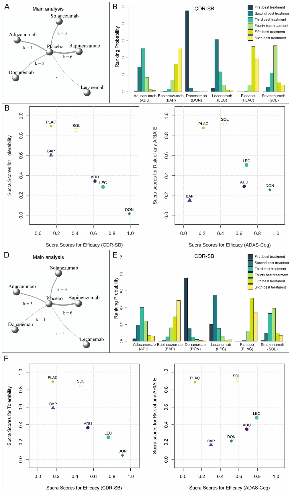
830 Figure 1. The results of Bayesian NMA for efficacy and safety of anti-amyloid 831 antibodies in Alzheimer’s disease in phase III randomized placebo-controlled clinical 832 trials. A, B and C correspond to the main analysis with all studies included, and D, E
