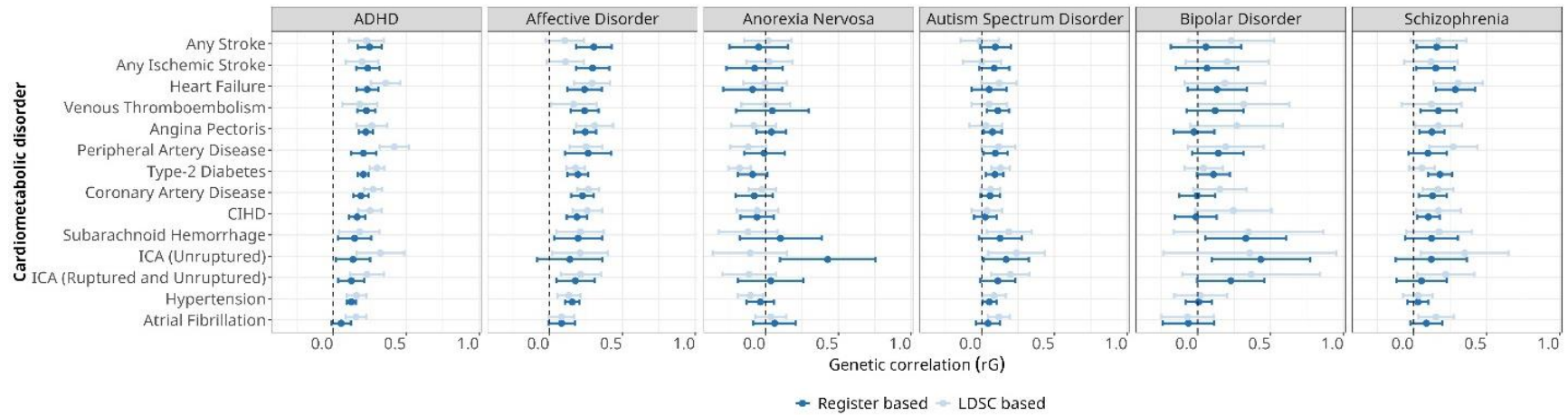
Supplementary figure S4: Comparison of the genetic correlations and 95% confidence intervals between mental- and cardiometabolic disorders calculated using register data ( r_g ) and LDSC ( r_{g\text{SNP}} ). ADHD = attention deficit/hyperactivity disorder, ICA = intracranial aneurysm, CIHD = chronic ischemic heart disease
