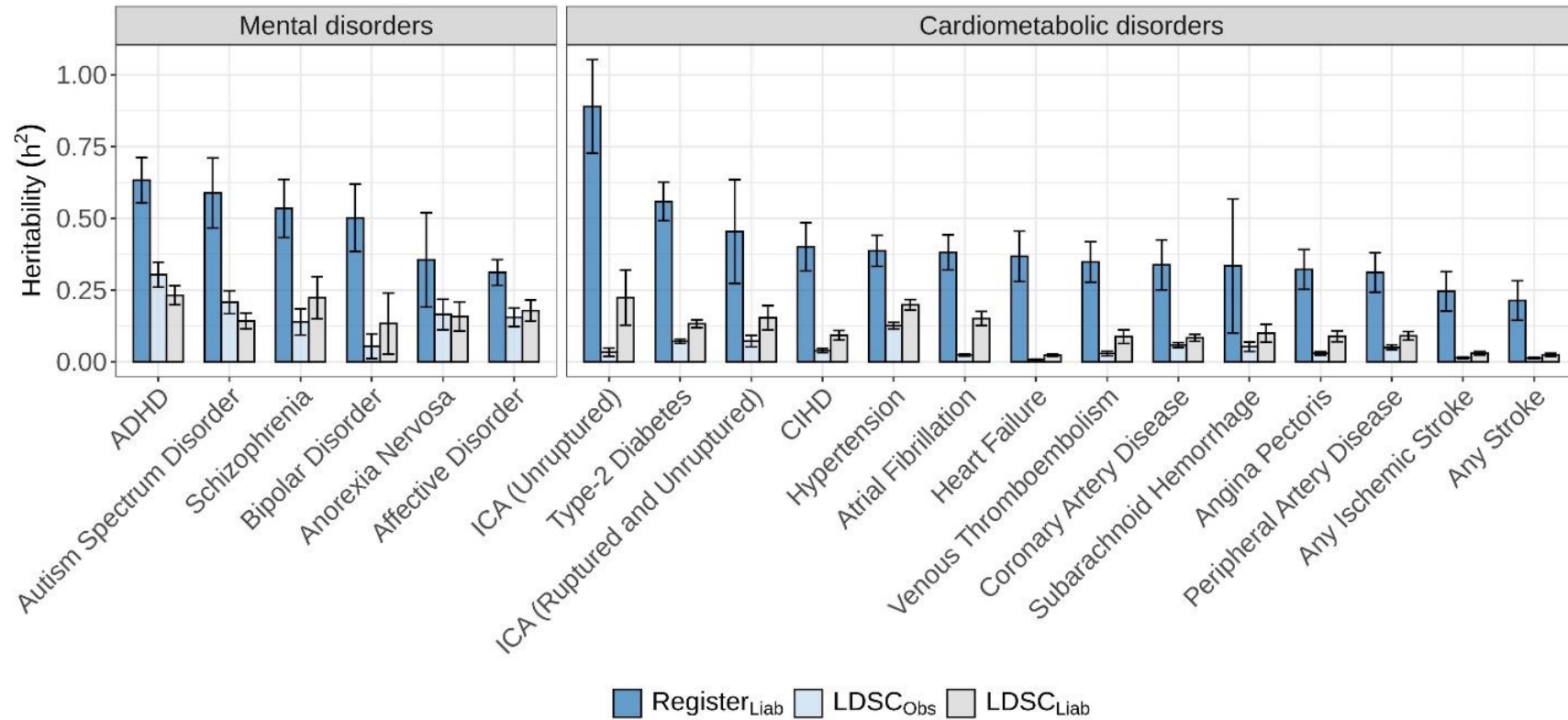
Supplementary figure S3: Narrow sense heritability ( h^2 ) estimates and 95% confidence intervals of mental- and cardiometabolic disorders using the Danish registers ( \text{Register}_{\text{Liab}} ) and LD-score regression on the observed ( \text{LDSC}_{\text{Obs}} ) and liability scale ( \text{LDSC}_{\text{Liab}} ). ADHD = attention deficit/hyperactivity disorder, ICA = intracranial aneurysm, CIHD = chronic ischemic heart disease
