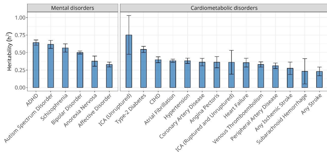
Figure 2: Meta-analysis of Danish and Swedish narrow sense heritability ( h^2 ) estimates and 95% confidence intervals of mental- and cardiometabolic disorders. ADHD = attention deficit/hyperactivity disorder, ICA = intracranial aneurysm, CIHD = chronic ischemic heart disease
