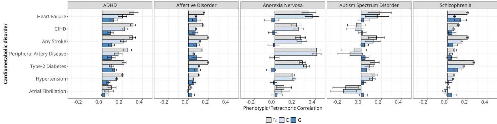
Figure 4: Quantification of the contribution of genetic (G) and the non-genetic (E) factors to the observed phenotypic correlation ( r_p ) between mental- and cardiometabolic disorders using register based genetic correlations ( r_g ) and heritability ( h^2 ) estimates. Estimates of r_p were selected from Momen et al. 1 .
