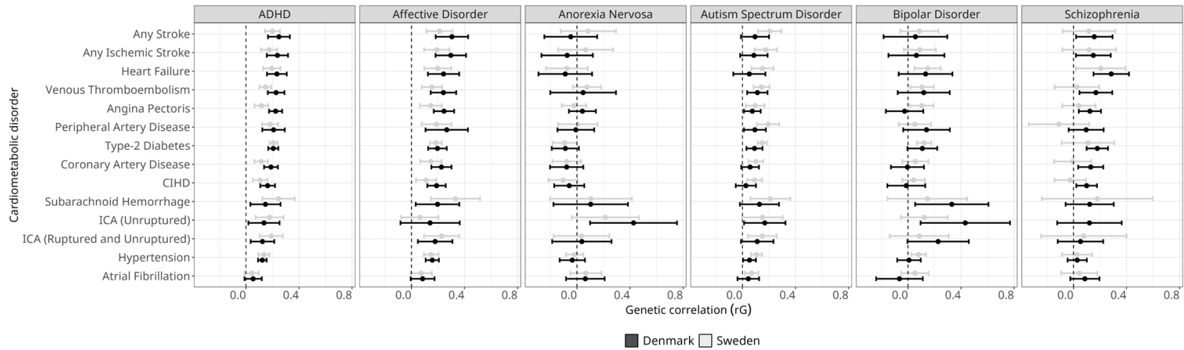
Supplementary figure S1: Comparison of Danish and Swedish register-based estimates and 95% confidence intervals for A.) heritability ( h^2 ) B.) genetic correlations ( r_G ). ADHD = attention deficit/hyperactivity disorder, ICA = intracranial aneurysm, CIHD = chronic ischemic heart disease
