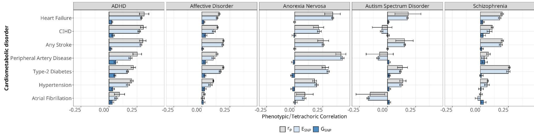
Supplementary figure S6: Quantification of the contribution of genetic ( G_{\text{SNP}} ) and the non-genetic ( E_{\text{SNP}} ) factors to the observed phenotypic correlation ( r_p ) between mental- and cardiometabolic disorders using LDSC based genetic correlations ( r_{g \text{ SNP}} ) and heritability ( h^2_{\text{SNP}} ) estimates. Estimates of r_p were selected from Momen et al. 1
