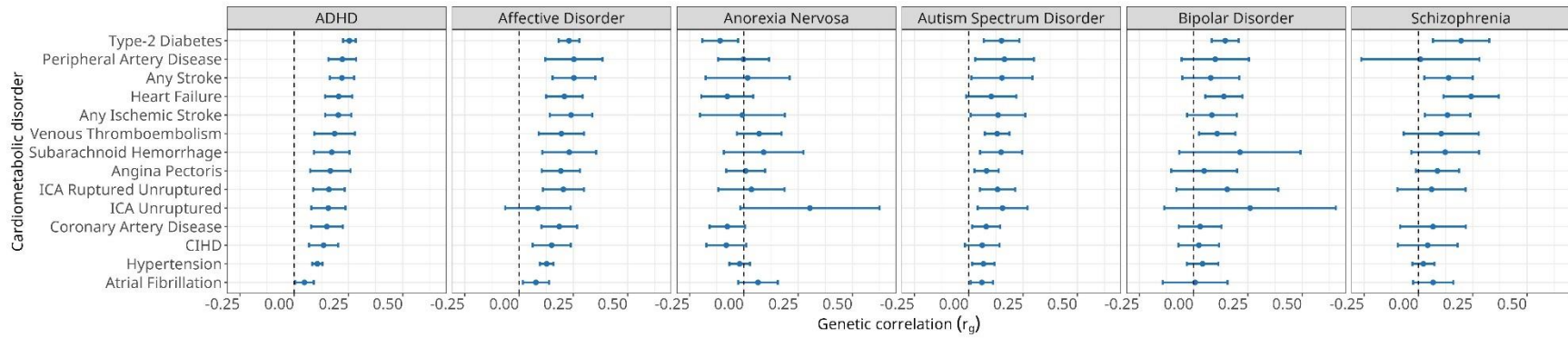
Figure 3: Meta-analysis of Danish and Swedish genetic correlations ( r_g ) estimates between mental- and cardiometabolic disorders and 95% confidence intervals calculated using national register data. ADHD = attention deficit/hyperactivity disorder, ICA = intracranial aneurysm, CIHD = chronic ischemic heart disease
