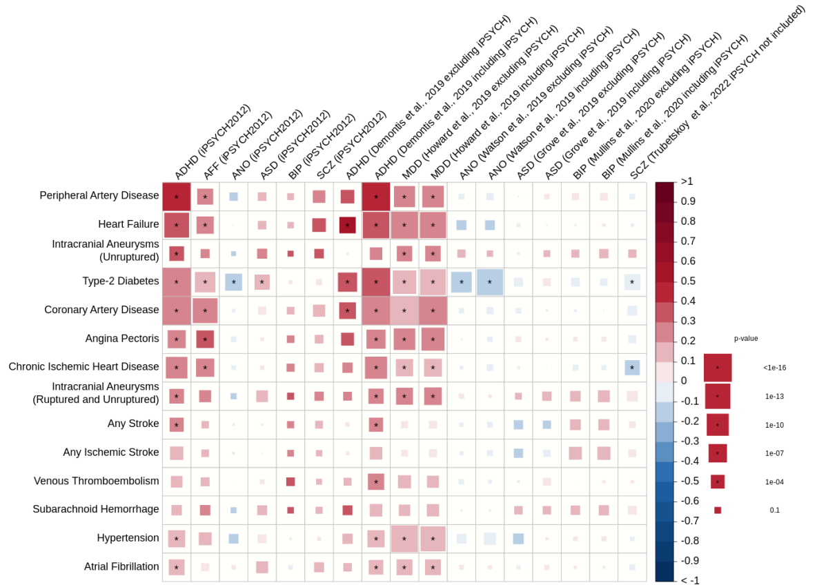
Supplementary figure S5: LDSC genetic correlations between six mental- and 14 cardiometabolic disorders. Genetic correlations ( r_{g\text{ SNP}} ) with standard error, and p-values. We repeated the analysis three times: using only iPSYCH samples and using the Psychiatric Genomics Consortium (PGC) meta-analysis including and excluding iPSYCH samples. Trubetskoy et al, 2022 did not contain iPSYCH samples. No PGC-AFF disorder GWAS meta-analysis exists therefore we used MDD as the next closest disorder.
