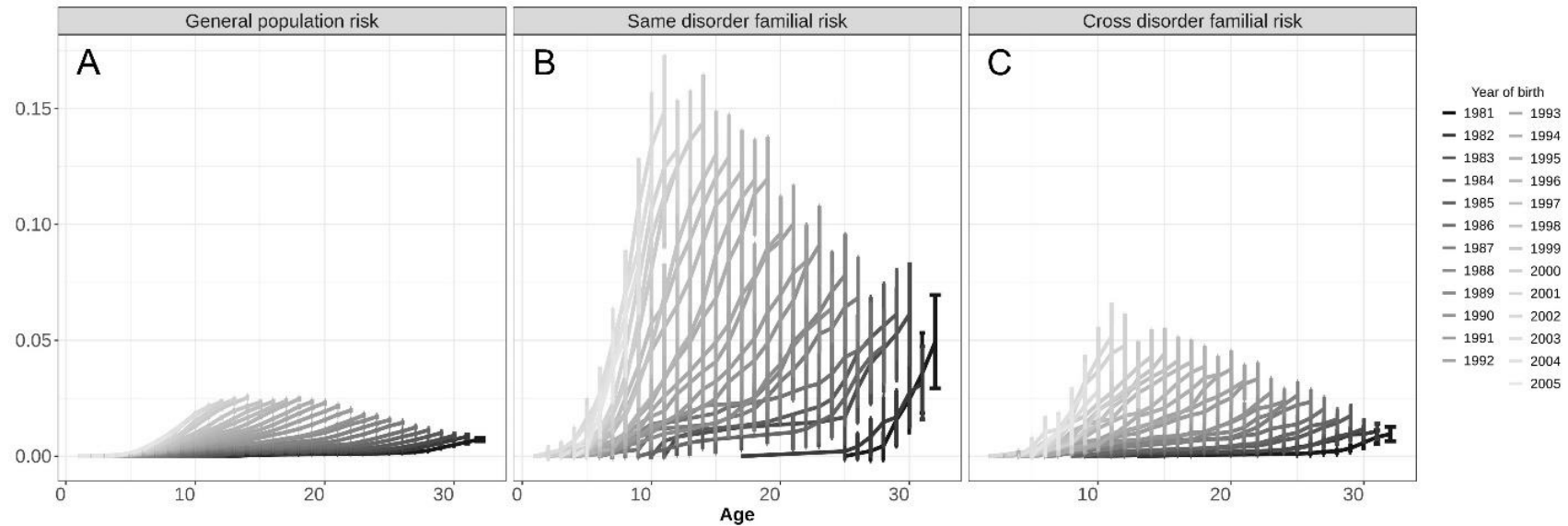
Figure 1: Cumulative incidences and 95% confidence intervals of ADHD for individuals born 1981-2005 using medical records up to 2012 stratified by year of birth. Cumulative incidences are shown for: A.) the general population, B.) individuals with at least one full-sibling diagnosed with ADHD, C.) individuals with at least one parent diagnosed with type-2 diabetes.
