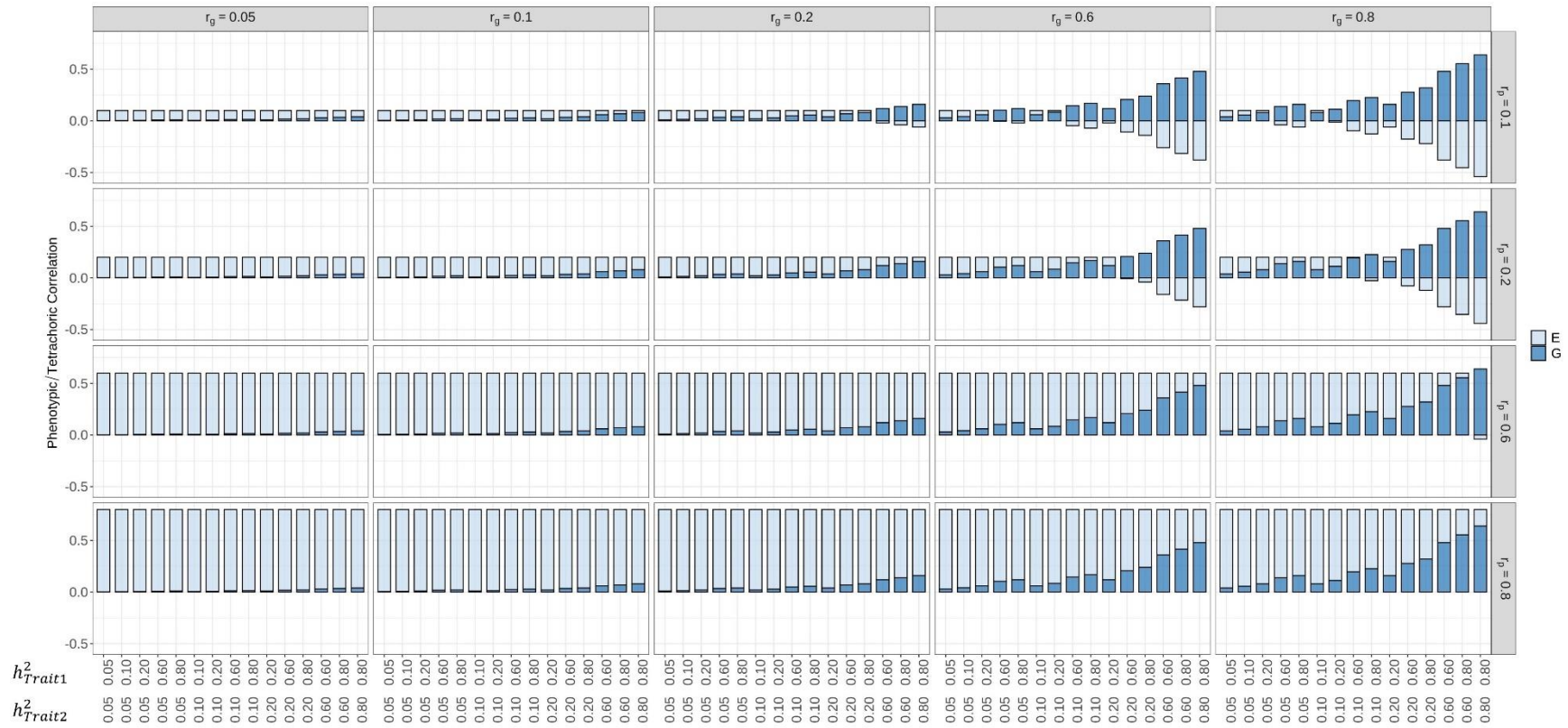
Figure 2: The effect of heritability ( h^2 ) and genetic correlation ( r_g ) size on the magnitude of the genetic (G) and non-genetic (E) contribution to the phenotypic correlation ( r_p ) between two traits. Phenotypic correlations ( r_p ) were derived using simulated hazard ratios (HZ) and prevalence's (Pr) of: r_p = 0.1 : HZ=1.28, Pr=0.05; r_p=0.2 : HZ=1.61, Pr=0.12; r_p=0.6 : HZ=4, Pr=0.2; r_p=0.8 : HZ=4, Pr=0.5.
