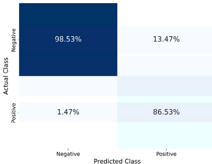
Figure 5. Confusion matrix of the XGBoost model.
