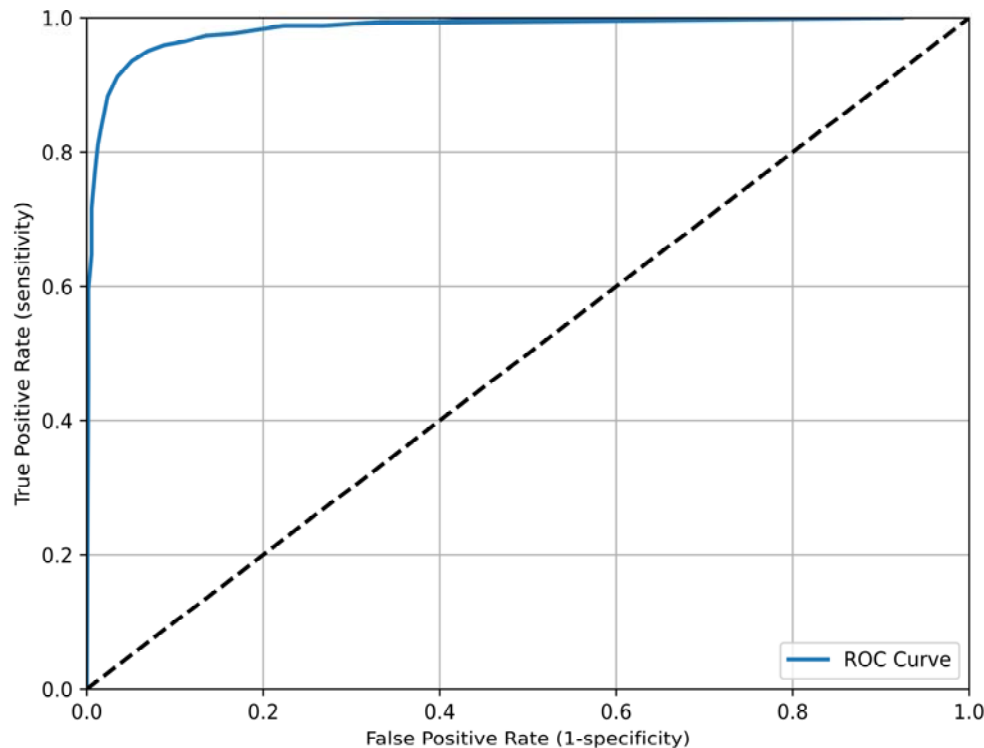
Figure 4. Receiver operating characteristics curve of the algorithm for hold-out test data predictions up to six hours before sepsis onset.
