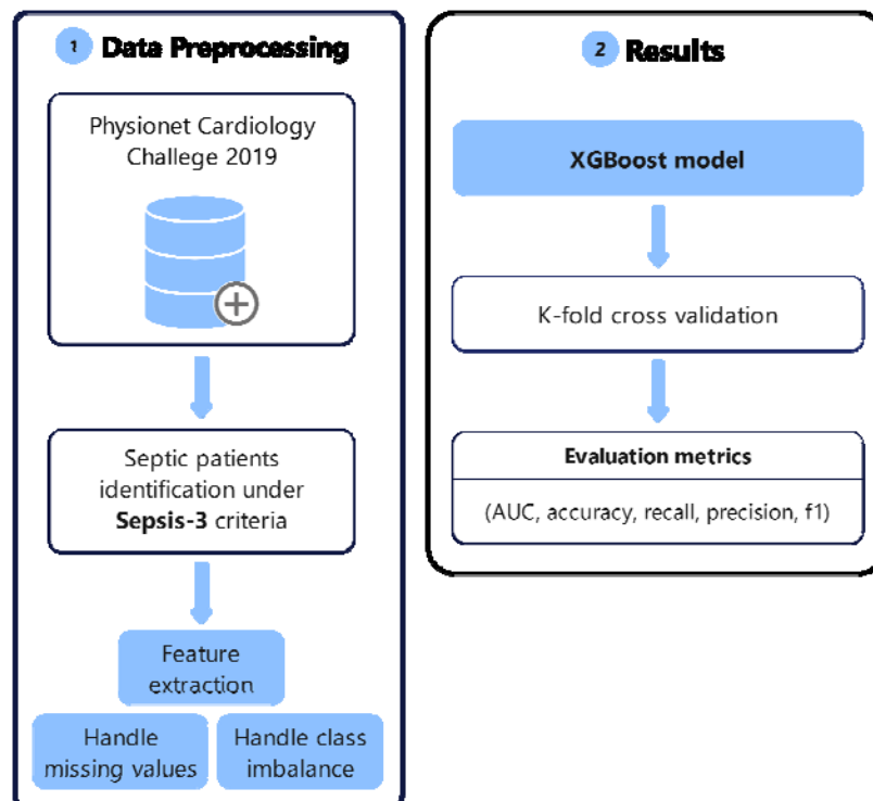
Figure 1. Flowchart of the proposed sepsis prediction workflow from preprocessing datasets to evaluating sepsis predictions using XGBoost.
