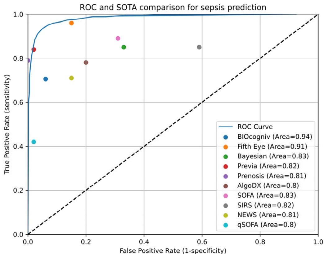
Figure 6. ROC curves of the VIOSync SPI model compared to SOTA model and scores for sepsis prediction onset.
