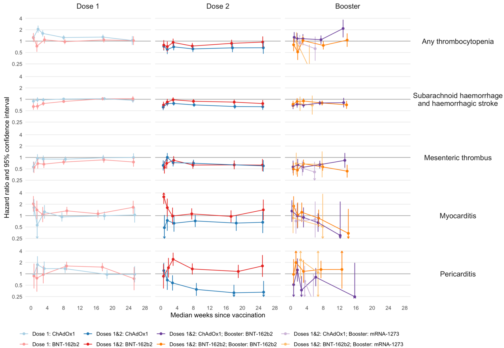
Figure 3: Associations of COVID-19 vaccination brand and dose with other cardiovascular events.
