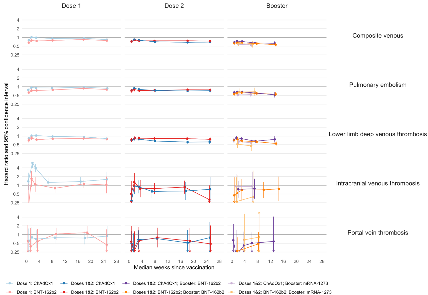
Figure 2: Associations of COVID-19 vaccination brand and dose with venous thromboses.
