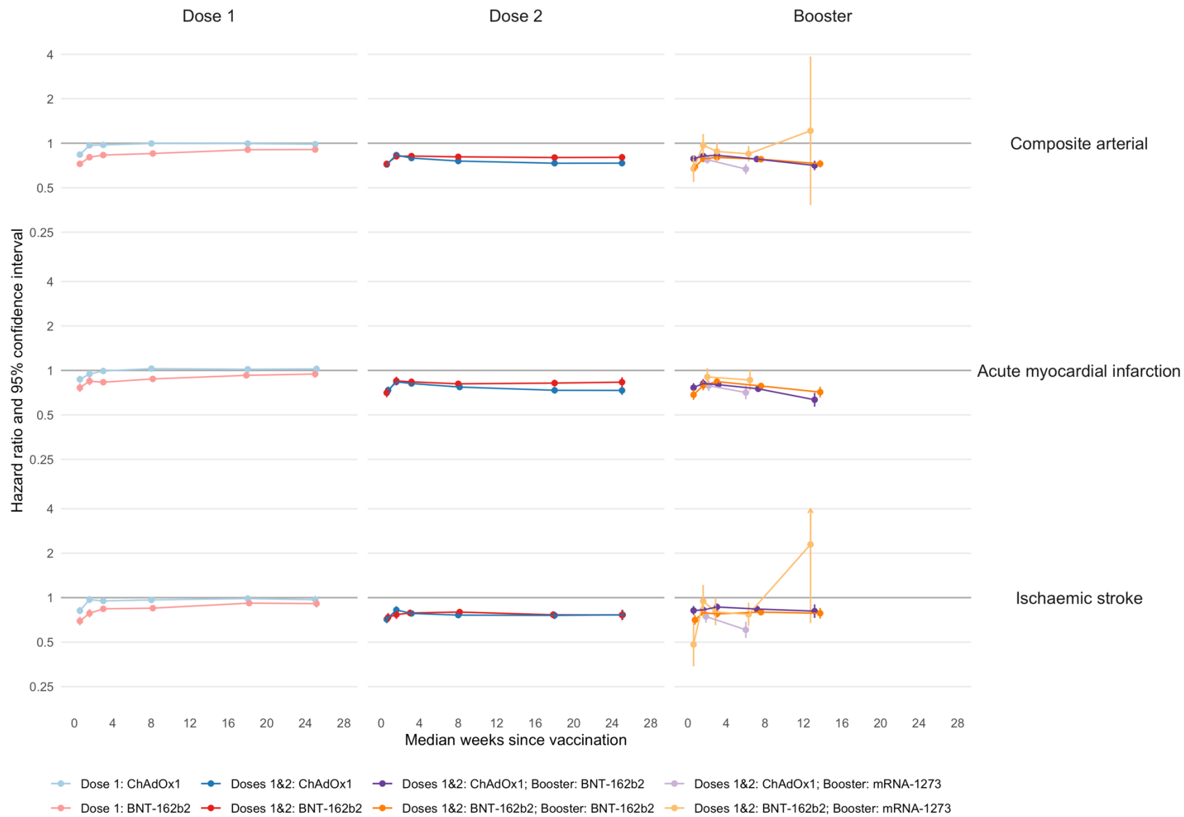
Figure 1: Associations of COVID-19 vaccination brand and dose with arterial thromboses
